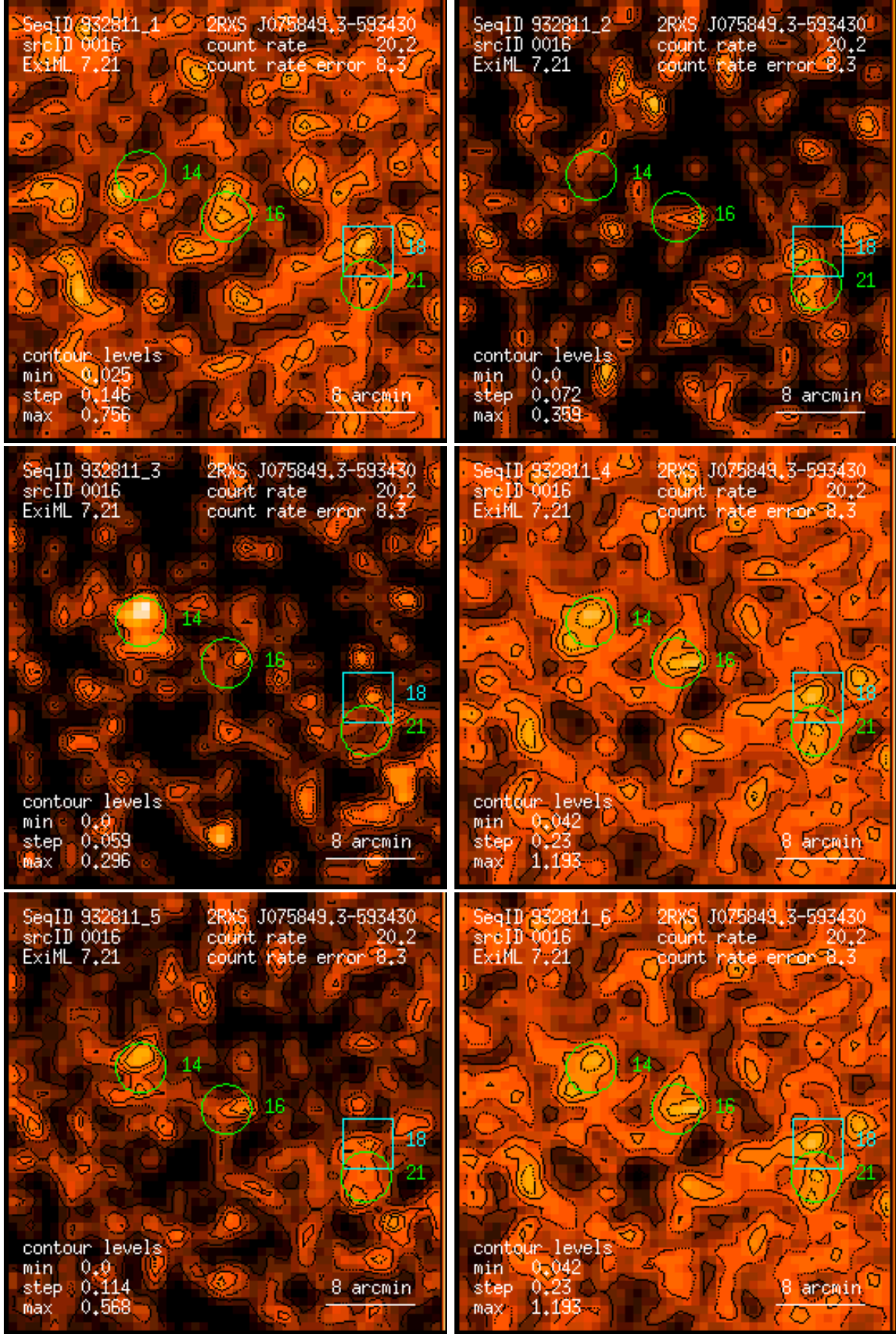
Figure 16: RASS 932811: detection 0016: band rate images, Gaussian filter: (1) PSPC channels 11 – 41, (2) 52 – 90, (3) 91 – 201, (4) 11 – 235, (5) 52 – 201, (6) 11 – 201. Broad band rates in counts/ks. Band rate contour levels in counts/ks/arcmin 2 .
