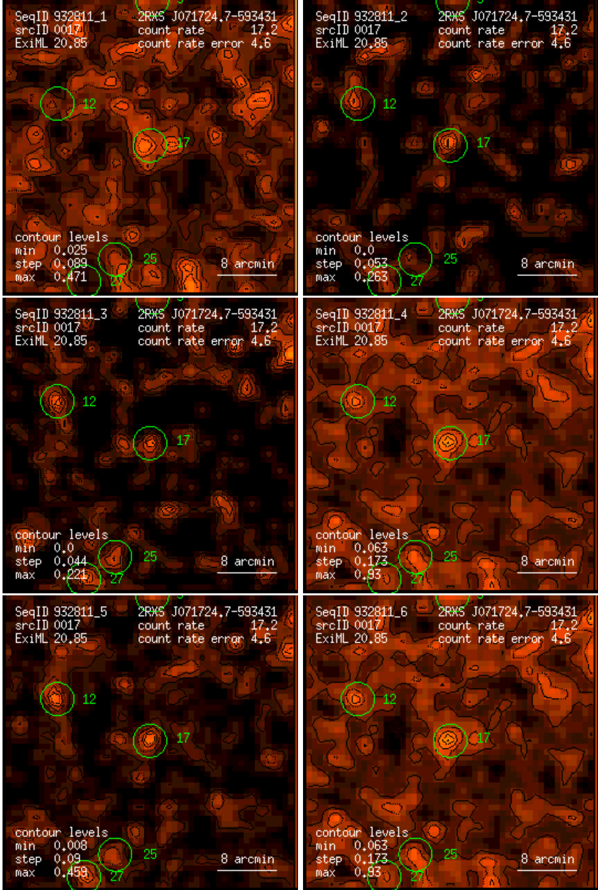
Figure 17: RASS 932811: detection 0017: band rate images, Gaussian filter: (1) PSPC channels 11 – 41, (2) 52 – 90, (3) 91 – 201, (4) 11 – 235, (5) 52 – 201, (6) 11 – 201. Broad band rates in counts/ks. Band rate contour levels in counts/ks/arcmin 2 .
