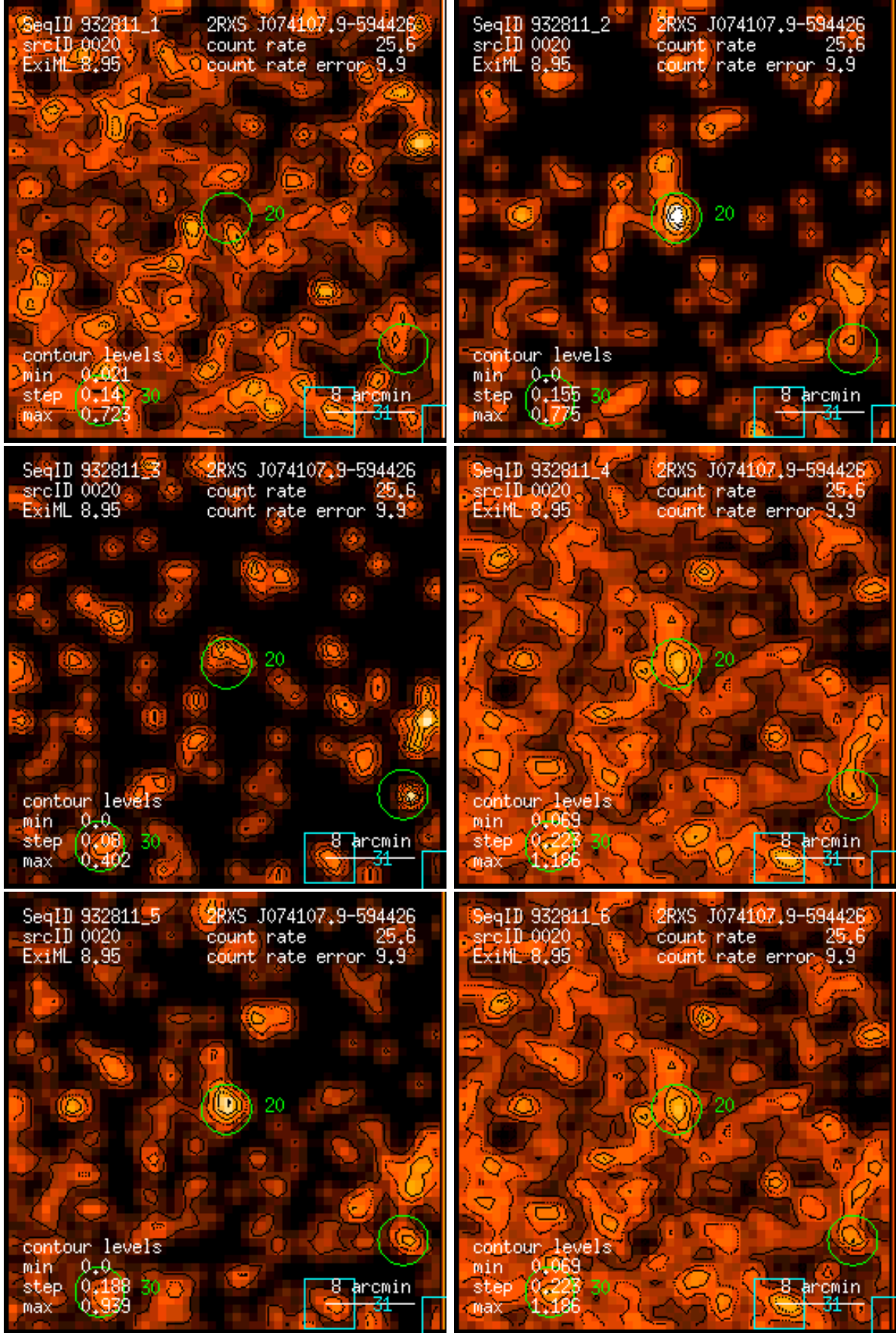
Figure 20: RASS 932811: detection 0020: band rate images, Gaussian filter: (1) PSPC channels 11 – 41, (2) 52 – 90, (3) 91 – 201, (4) 11 – 235, (5) 52 – 201, (6) 11 – 201. Broad band rates in counts/ks. Band rate contour levels in counts/ks/arcmin 2 .
