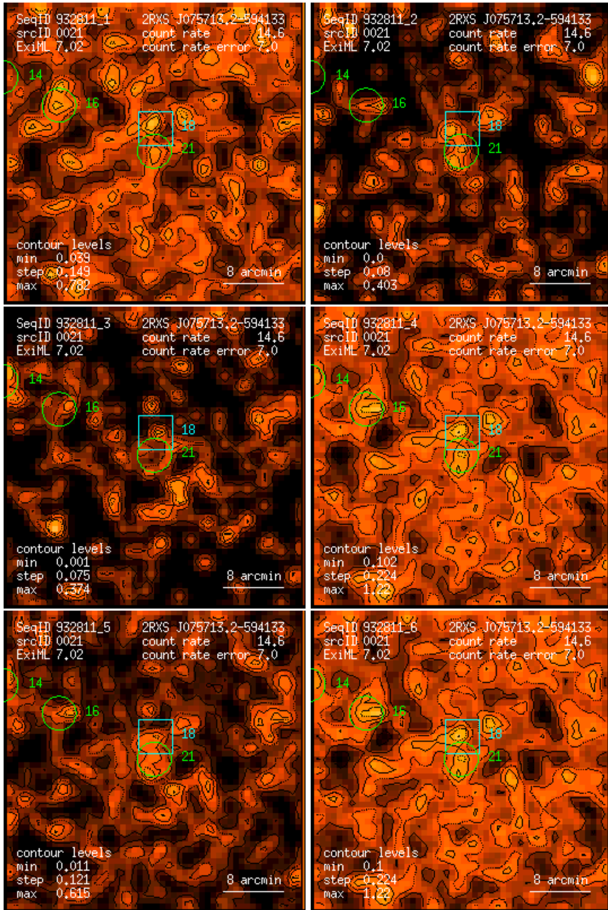
Figure 21: RASS 932811: detection 0021: band rate images, Gaussian filter: (1) PSPC channels 11 – 41, (2) 52 – 90, (3) 91 – 201, (4) 11 – 235, (5) 52 – 201, (6) 11 – 201. Broad band rates in counts/ks. Band rate contour levels in counts/ks/arcmin 2 .
