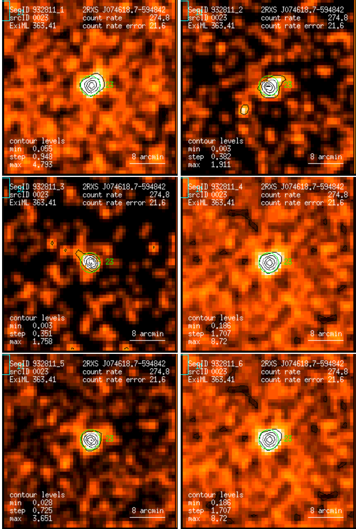
Figure 23: RASS 932811: detection 0023: band rate images, Gaussian filter: (1) PSPC channels 11 – 41, (2) 52 – 90, (3) 91 – 201, (4) 11 – 235, (5) 52 – 201, (6) 11 – 201. Broad band rates in counts/ks. Band rate contour levels in counts/ks/arcmin 2 .
