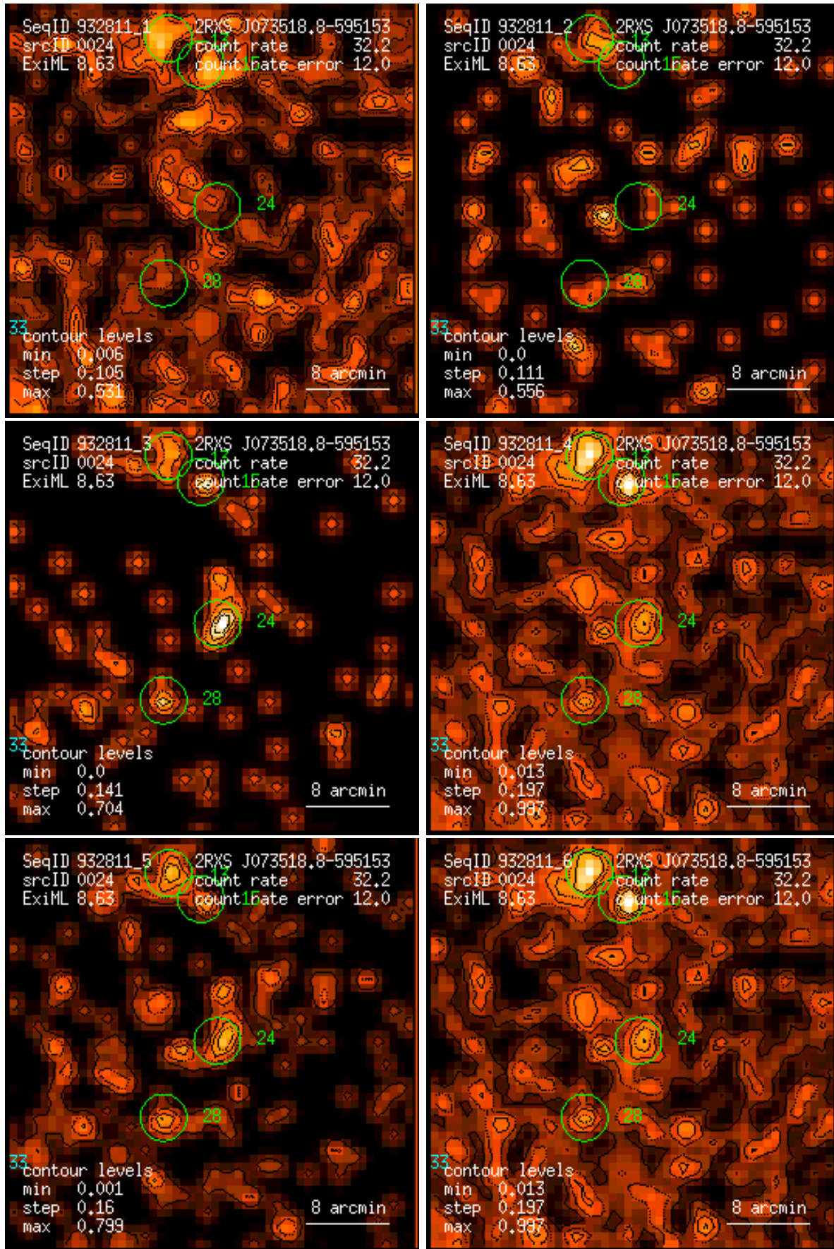
Figure 24: RASS 932811: detection 0024: band rate images, Gaussian filter: (1) PSPC channels 11 – 41, (2) 52 – 90, (3) 91 – 201, (4) 11 – 235, (5) 52 – 201, (6) 11 – 201. Broad band rates in counts/ks. Band rate contour levels in counts/ks/arcmin 2 .
