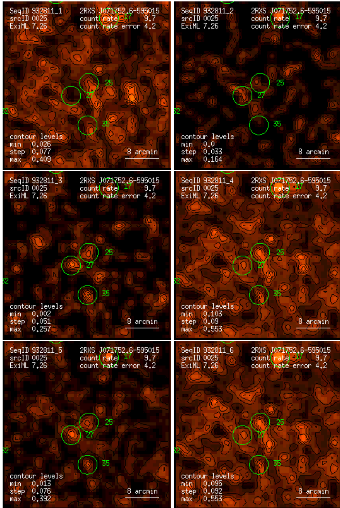
Figure 25: RASS 932811: detection 0025: band rate images, Gaussian filter: (1) PSPC channels 11 – 41, (2) 52 – 90, (3) 91 – 201, (4) 11 – 235, (5) 52 – 201, (6) 11 – 201. Broad band rates in counts/ks. Band rate contour levels in counts/ks/arcmin 2 .
