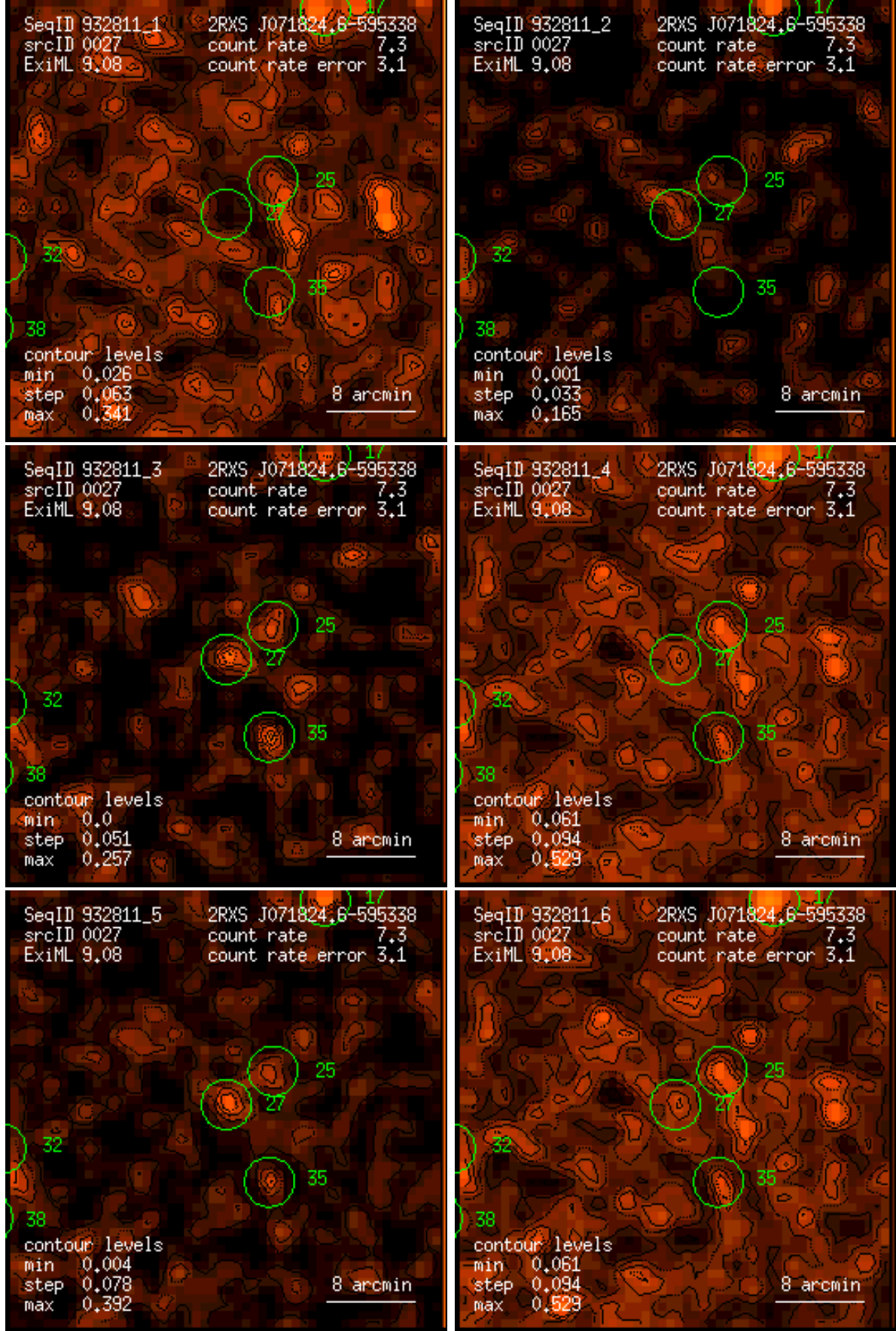
Figure 27: RASS 932811: detection 0027: band rate images, Gaussian filter: (1) PSPC channels 11 – 41, (2) 52 – 90, (3) 91 – 201, (4) 11 – 235, (5) 52 – 201, (6) 11 – 201. Broad band rates in counts/ks. Band rate contour levels in counts/ks/arcmin 2 .
