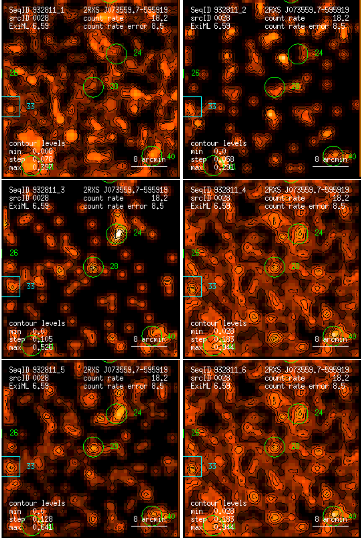
Figure 28: RASS 932811: detection 0028: band rate images, Gaussian filter: (1) PSPC channels 11 – 41, (2) 52 – 90, (3) 91 – 201, (4) 11 – 235, (5) 52 – 201, (6) 11 – 201. Broad band rates in counts/ks. Band rate contour levels in counts/ks/arcmin 2 .
