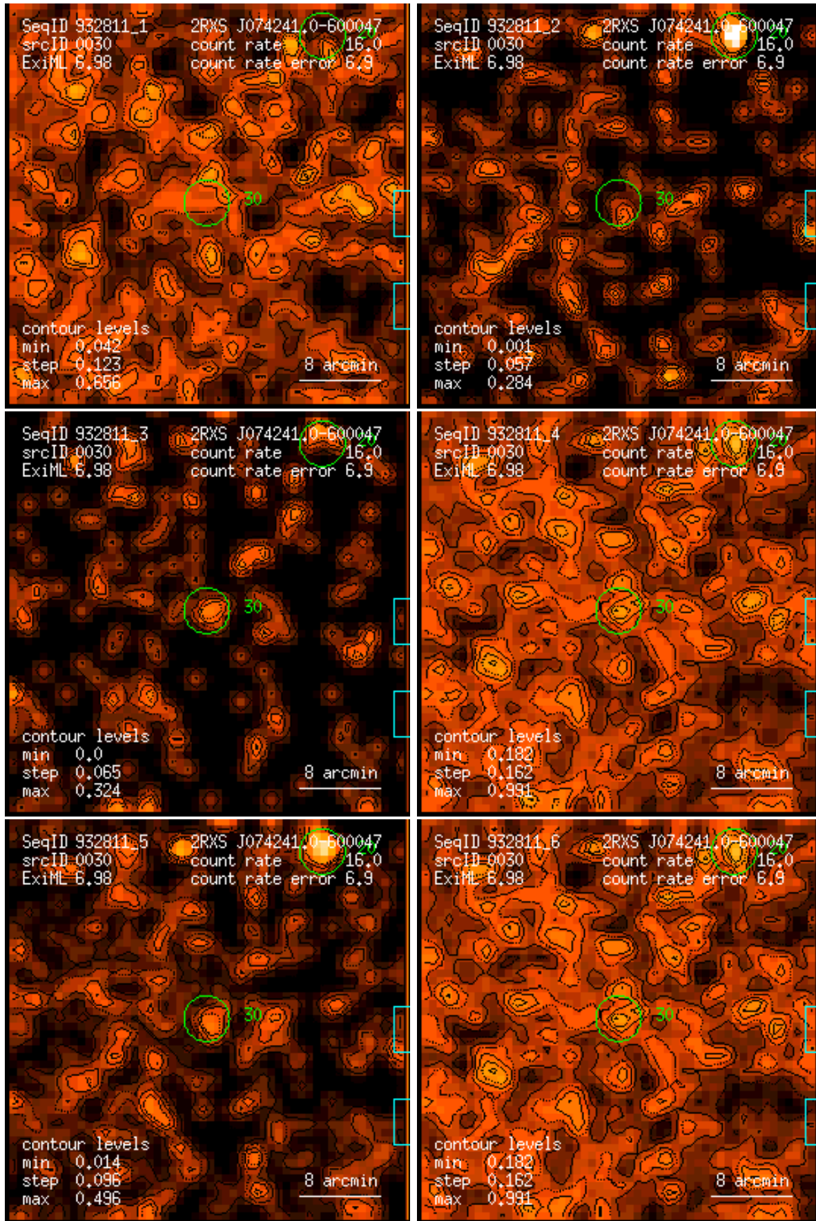
Figure 30: RASS 932811: detection 0030: band rate images, Gaussian filter: (1) PSPC channels 11 – 41, (2) 52 – 90, (3) 91 – 201, (4) 11 – 235, (5) 52 – 201, (6) 11 – 201. Broad band rates in counts/ks. Band rate contour levels in counts/ks/arcmin 2 .
