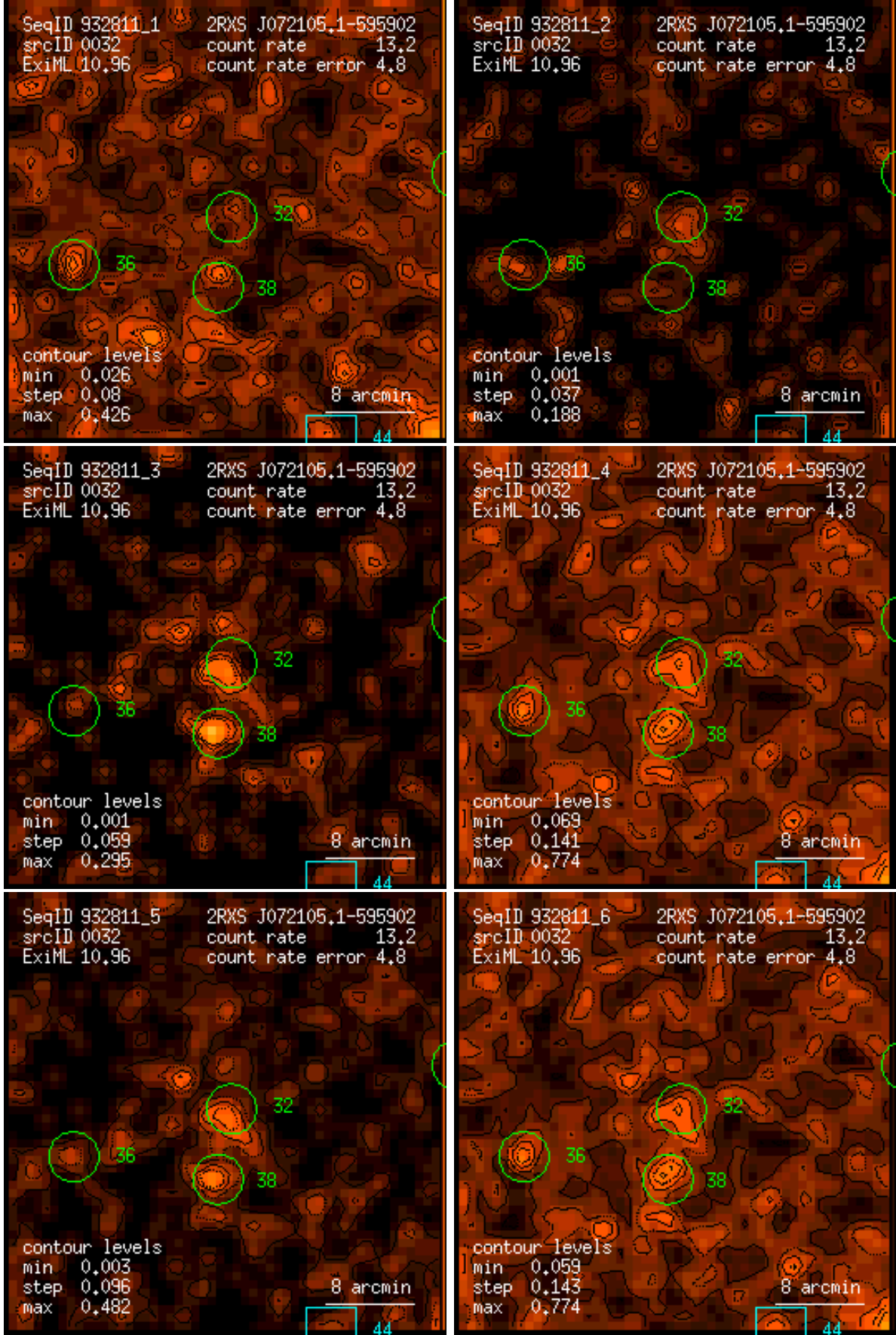
Figure 32: RASS 932811: detection 0032: band rate images, Gaussian filter: (1) PSPC channels 11 – 41, (2) 52 – 90, (3) 91 – 201, (4) 11 – 235, (5) 52 – 201, (6) 11 – 201. Broad band rates in counts/ks. Band rate contour levels in counts/ks/arcmin 2 .
