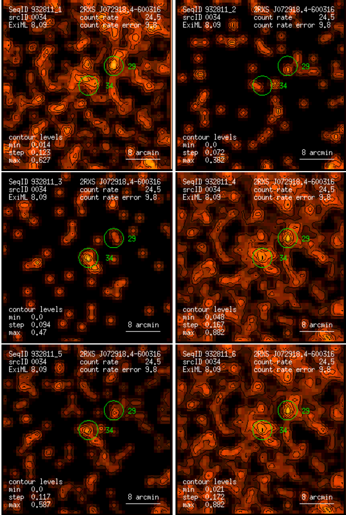
Figure 34: RASS 932811: detection 0034: band rate images, Gaussian filter: (1) PSPC channels 11 – 41, (2) 52 – 90, (3) 91 – 201, (4) 11 – 235, (5) 52 – 201, (6) 11 – 201. Broad band rates in counts/ks. Band rate contour levels in counts/ks/arcmin 2 .
