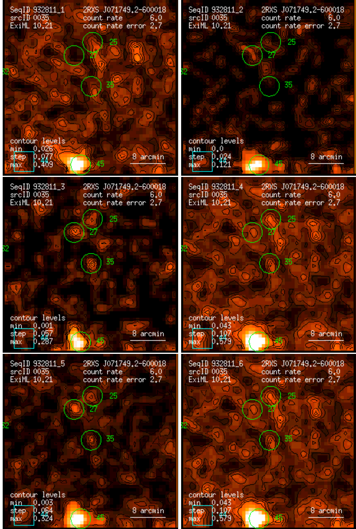
Figure 35: RASS 932811: detection 0035: band rate images, Gaussian filter: (1) PSPC channels 11 – 41, (2) 52 – 90, (3) 91 – 201, (4) 11 – 235, (5) 52 – 201, (6) 11 – 201. Broad band rates in counts/ks. Band rate contour levels in counts/ks/arcmin 2 .
