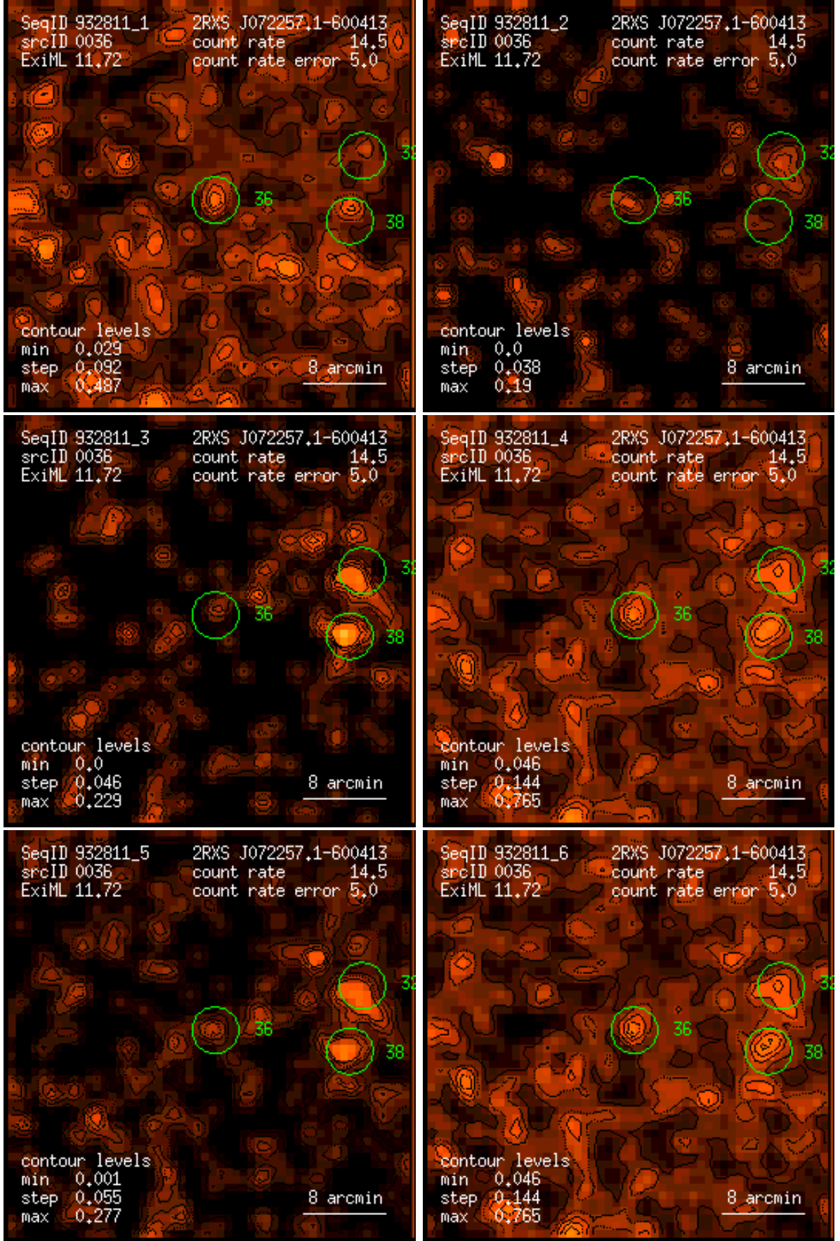
Figure 36: RASS 932811: detection 0036: band rate images, Gaussian filter: (1) PSPC channels 11 – 41, (2) 52 – 90, (3) 91 – 201, (4) 11 – 235, (5) 52 – 201, (6) 11 – 201. Broad band rates in counts/ks. Band rate contour levels in counts/ks/arcmin 2 .
