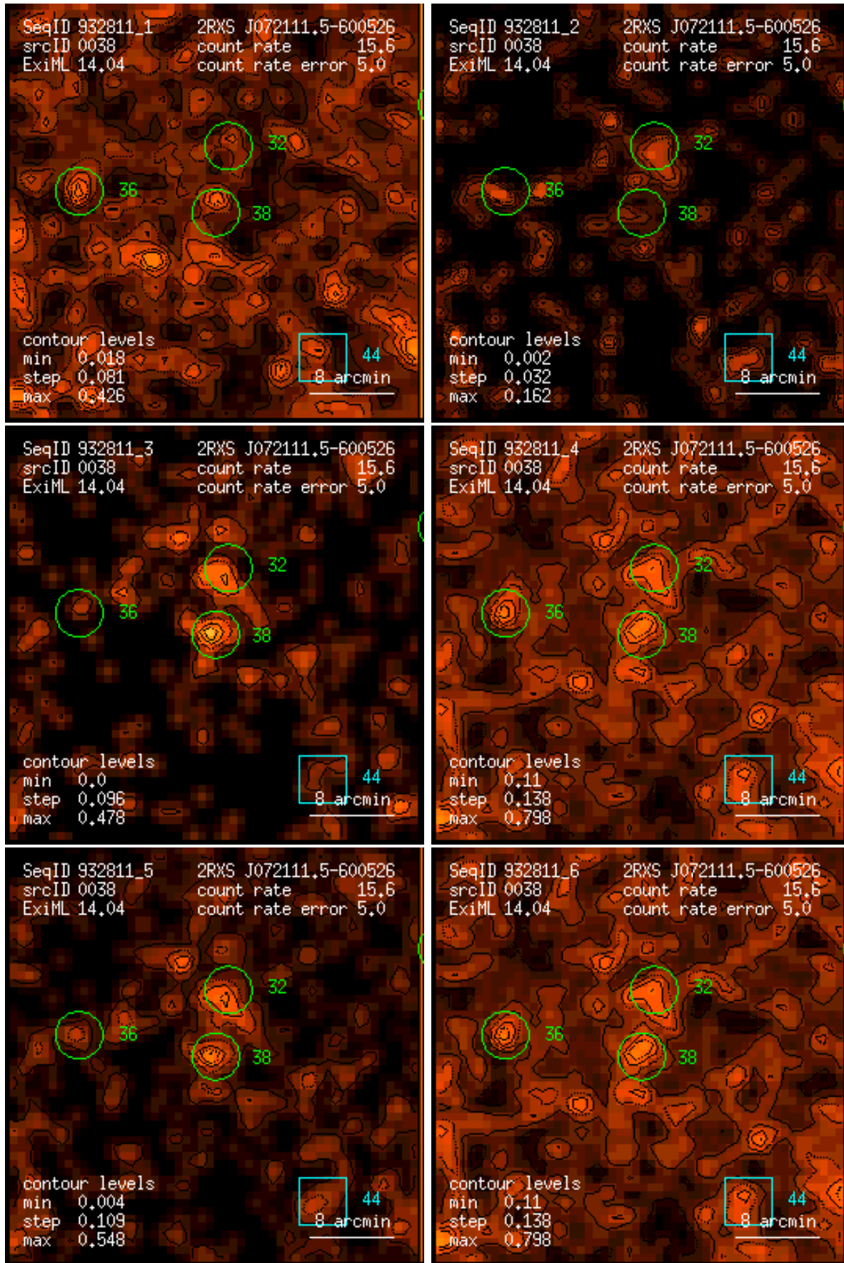
Figure 38: RASS 932811: detection 0038: band rate images, Gaussian filter: (1) PSPC channels 11 – 41, (2) 52 – 90, (3) 91 – 201, (4) 11 – 235, (5) 52 – 201, (6) 11 – 201. Broad band rates in counts/ks. Band rate contour levels in counts/ks/arcmin 2 .
