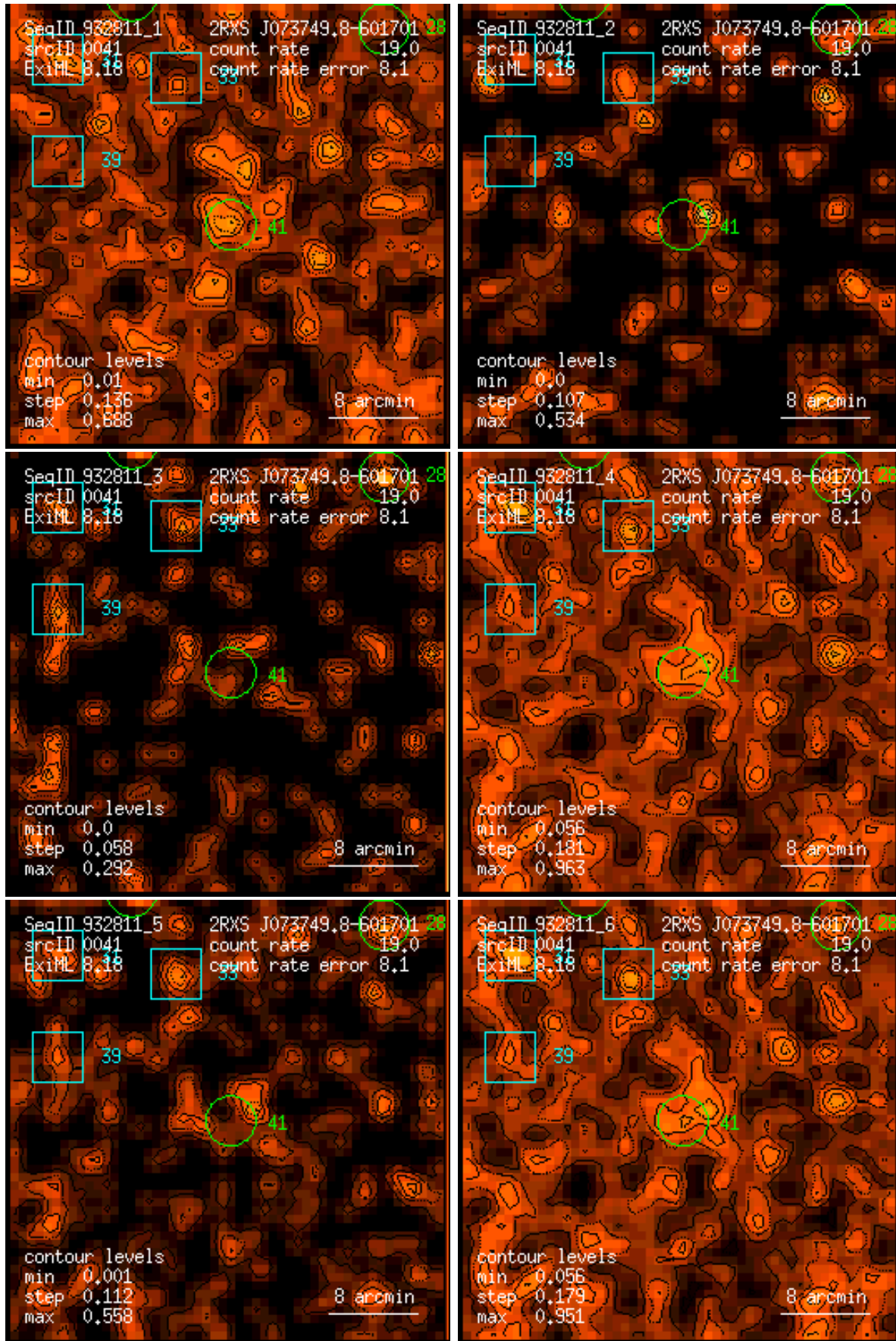
Figure 41: RASS 932811: detection 0041: band rate images, Gaussian filter: (1) PSPC channels 11 – 41, (2) 52 – 90, (3) 91 – 201, (4) 11 – 235, (5) 52 – 201, (6) 11 – 201. Broad band rates in counts/ks. Band rate contour levels in counts/ks/arcmin 2 .
