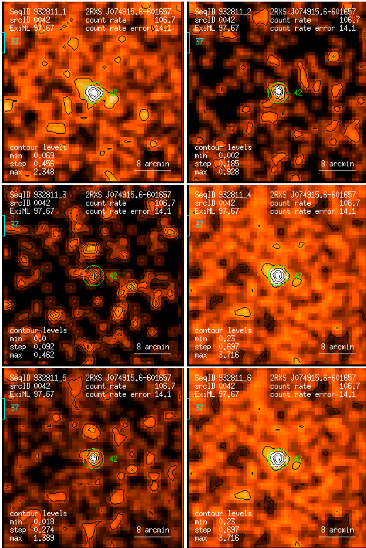
Figure 42: RASS 932811: detection 0042: band rate images, Gaussian filter: (1) PSPC channels 11 – 41, (2) 52 – 90, (3) 91 – 201, (4) 11 – 235, (5) 52 – 201, (6) 11 – 201. Broad band rates in counts/ks. Band rate contour levels in counts/ks/arcmin 2 .
