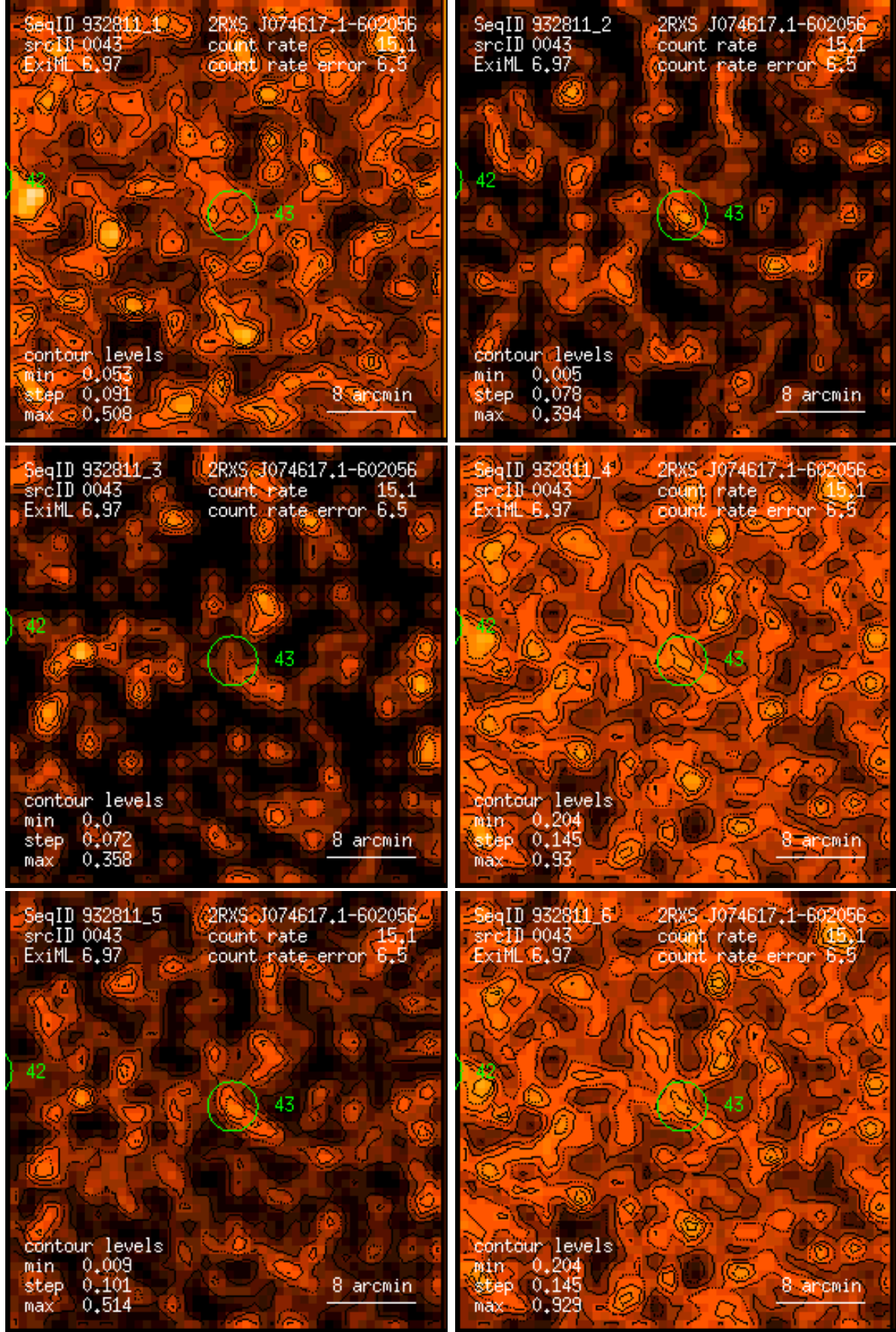
Figure 43: RASS 932811: detection 0043: band rate images, Gaussian filter: (1) PSPC channels 11 – 41, (2) 52 – 90, (3) 91 – 201, (4) 11 – 235, (5) 52 – 201, (6) 11 – 201. Broad band rates in counts/ks. Band rate contour levels in counts/ks/arcmin 2 .
