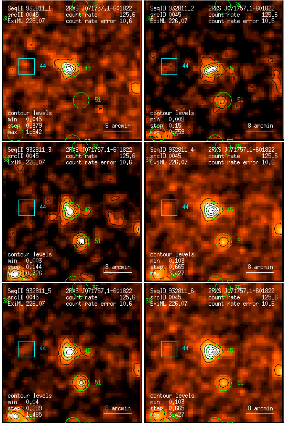
Figure 45: RASS 932811: detection 0045: band rate images, Gaussian filter: (1) PSPC channels 11 – 41, (2) 52 – 90, (3) 91 – 201, (4) 11 – 235, (5) 52 – 201, (6) 11 – 201. Broad band rates in counts/ks. Band rate contour levels in counts/ks/arcmin 2 .
