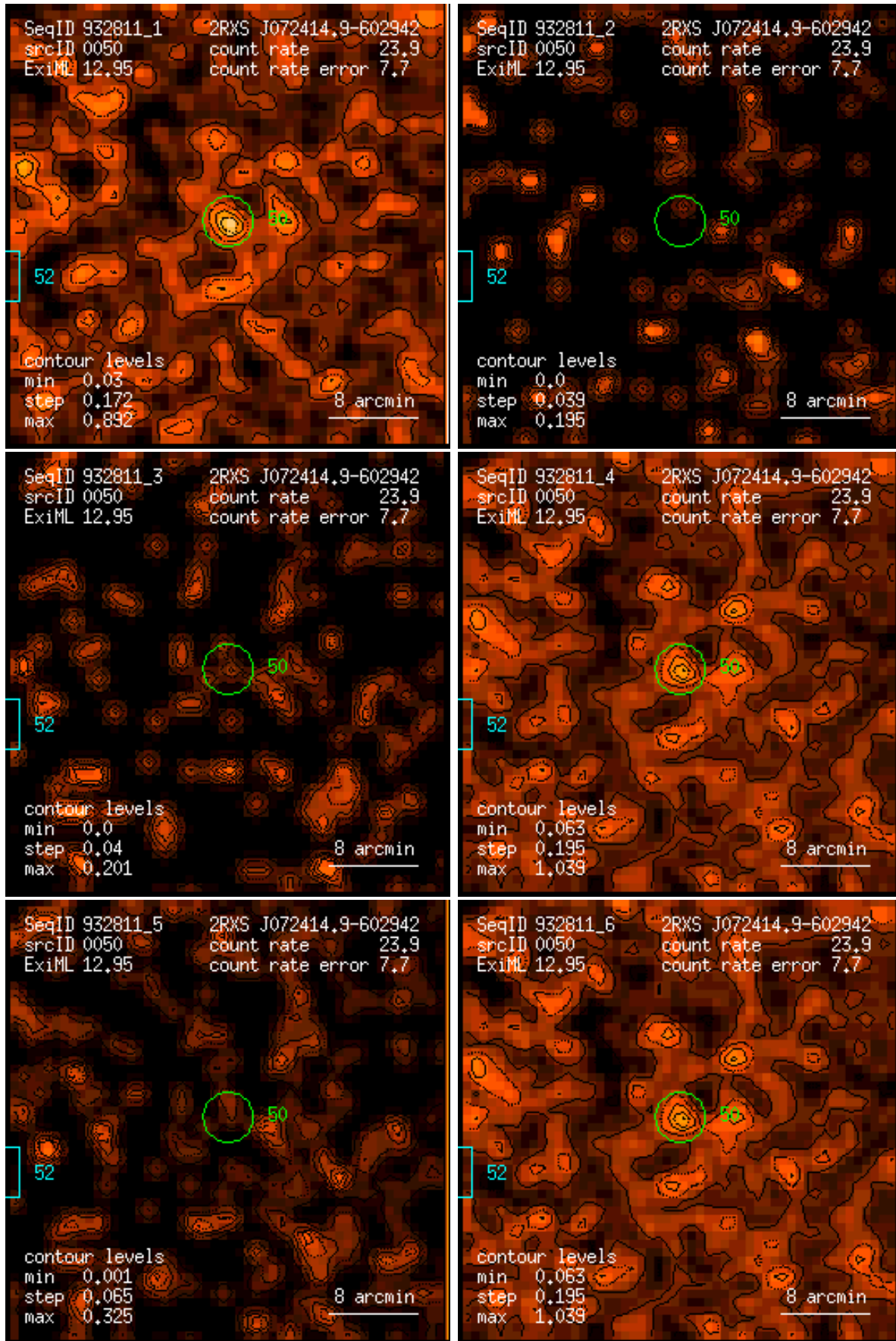
Figure 50: RASS 932811: detection 0050: band rate images, Gaussian filter: (1) PSPC channels 11 – 41, (2) 52 – 90, (3) 91 – 201, (4) 11 – 235, (5) 52 – 201, (6) 11 – 201. Broad band rates in counts/ks. Band rate contour levels in counts/ks/arcmin 2 .
