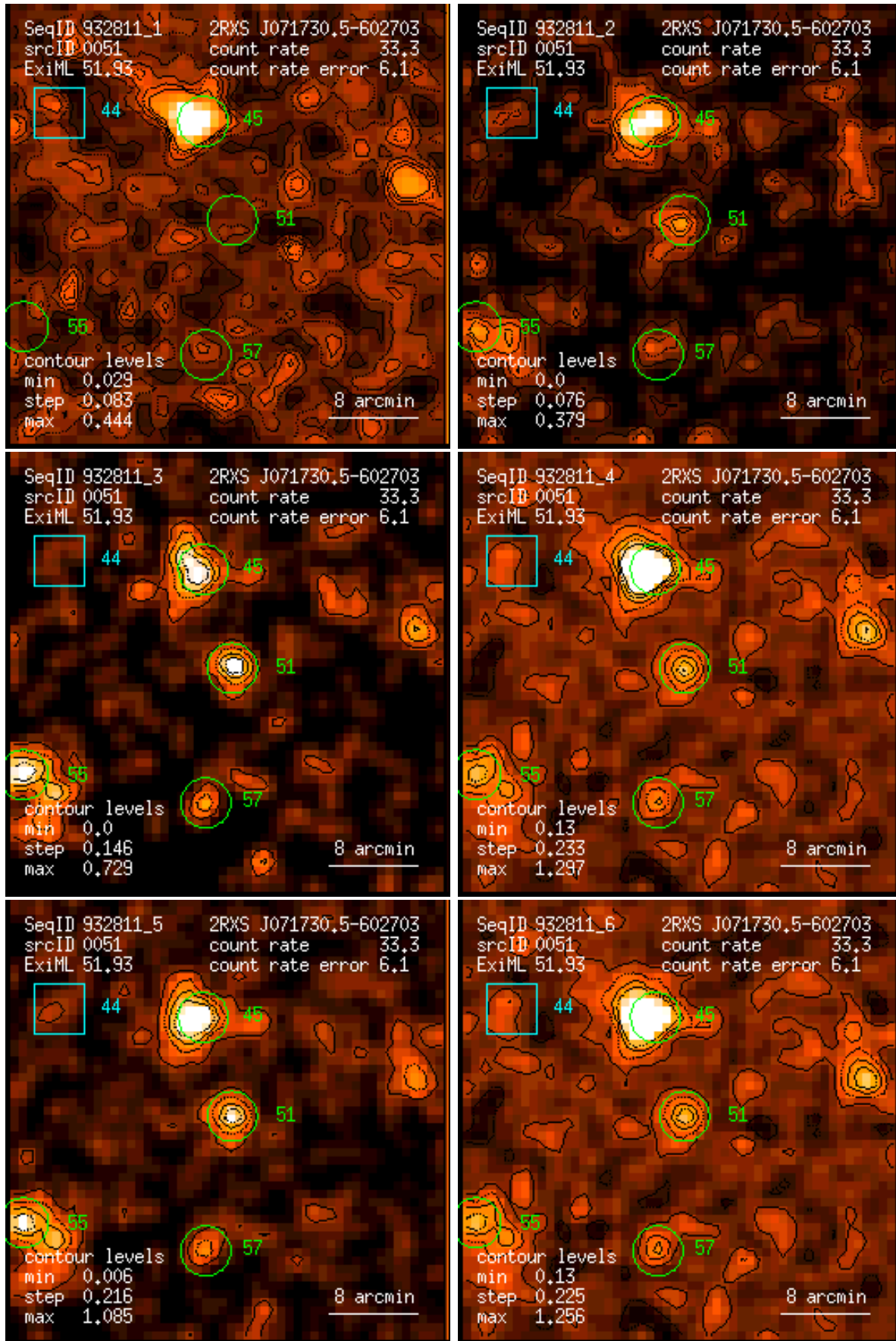
Figure 51: RASS 932811: detection 0051: band rate images, Gaussian filter: (1) PSPC channels 11 – 41, (2) 52 – 90, (3) 91 – 201, (4) 11 – 235, (5) 52 – 201, (6) 11 – 201. Broad band rates in counts/ks. Band rate contour levels in counts/ks/arcmin 2 .
