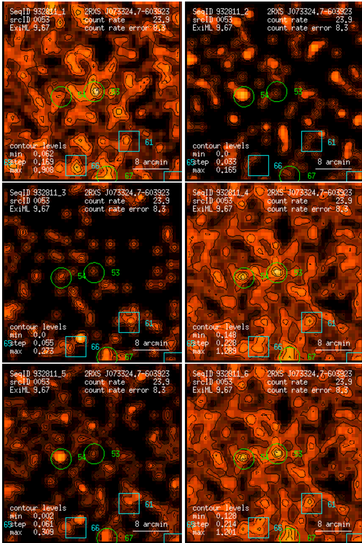
Figure 53: RASS 932811: detection 0053: band rate images, Gaussian filter: (1) PSPC channels 11 – 41, (2) 52 – 90, (3) 91 – 201, (4) 11 – 235, (5) 52 – 201, (6) 11 – 201. Broad band rates in counts/ks. Band rate contour levels in counts/ks/arcmin 2 .
