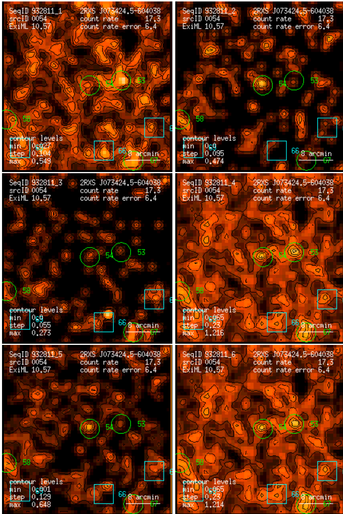
Figure 54: RASS 932811: detection 0054: band rate images, Gaussian filter: (1) PSPC channels 11 – 41, (2) 52 – 90, (3) 91 – 201, (4) 11 – 235, (5) 52 – 201, (6) 11 – 201. Broad band rates in counts/ks. Band rate contour levels in counts/ks/arcmin 2 .
