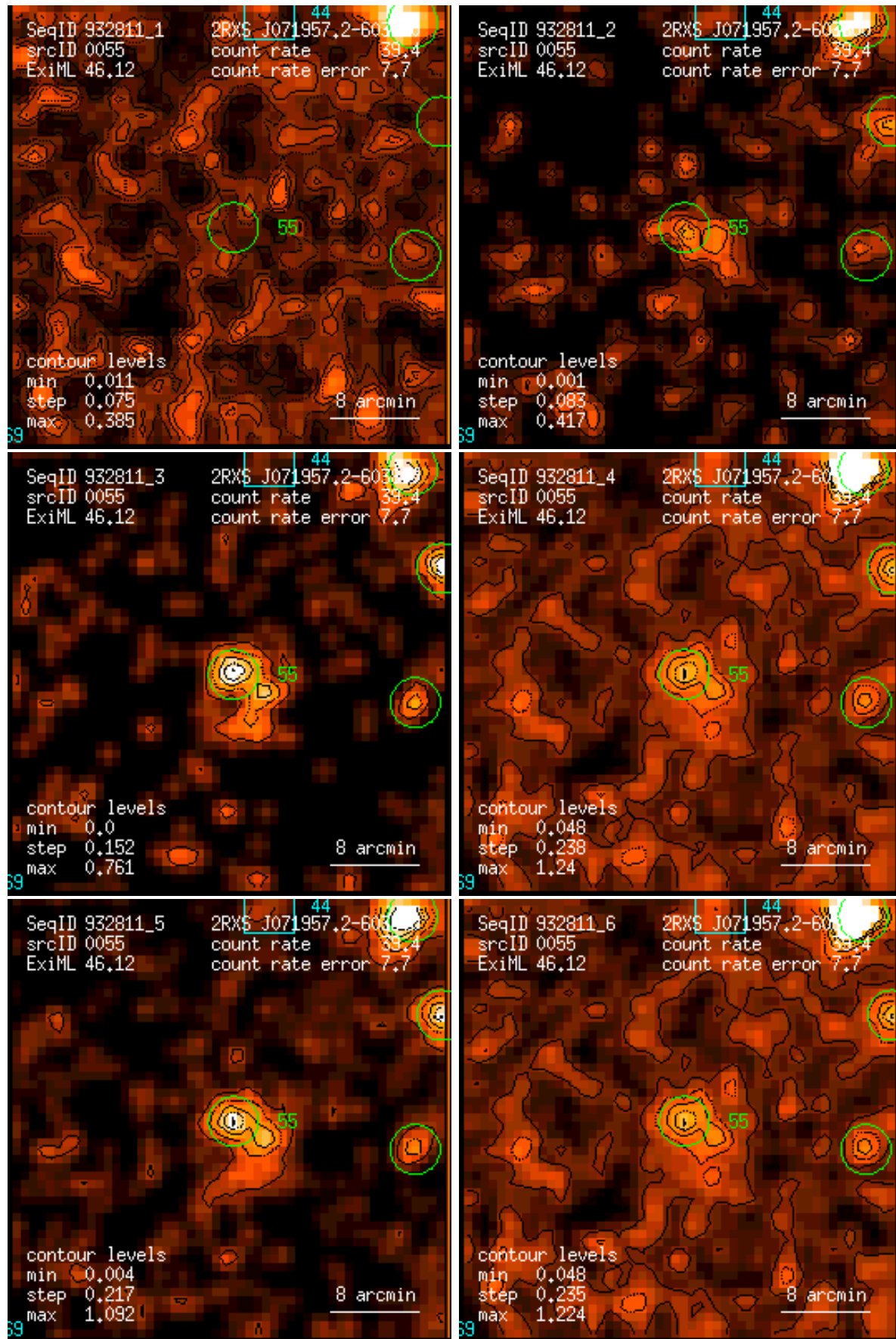
Figure 55: RASS 932811: detection 0055: band rate images, Gaussian filter: (1) PSPC channels 11 – 41, (2) 52 – 90, (3) 91 – 201, (4) 11 – 235, (5) 52 – 201, (6) 11 – 201. Broad band rates in counts/ks. Band rate contour levels in counts/ks/arcmin 2 .
