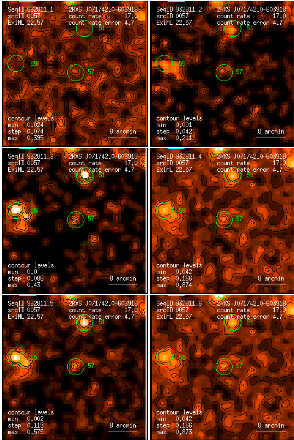
Figure 57: RASS 932811: detection 0057: band rate images, Gaussian filter: (1) PSPC channels 11 – 41, (2) 52 – 90, (3) 91 – 201, (4) 11 – 235, (5) 52 – 201, (6) 11 – 201. Broad band rates in counts/ks. Band rate contour levels in counts/ks/arcmin 2 .
