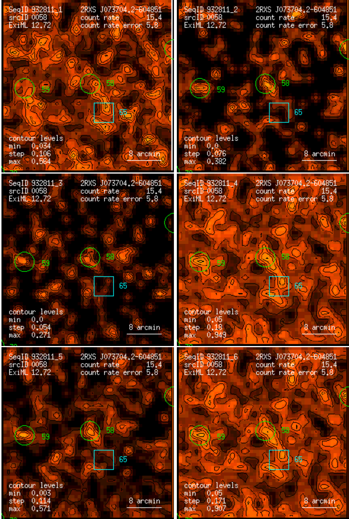
Figure 58: RASS 932811: detection 0058: band rate images, Gaussian filter: (1) PSPC channels 11 – 41, (2) 52 – 90, (3) 91 – 201, (4) 11 – 235, (5) 52 – 201, (6) 11 – 201. Broad band rates in counts/ks. Band rate contour levels in counts/ks/arcmin 2 .
