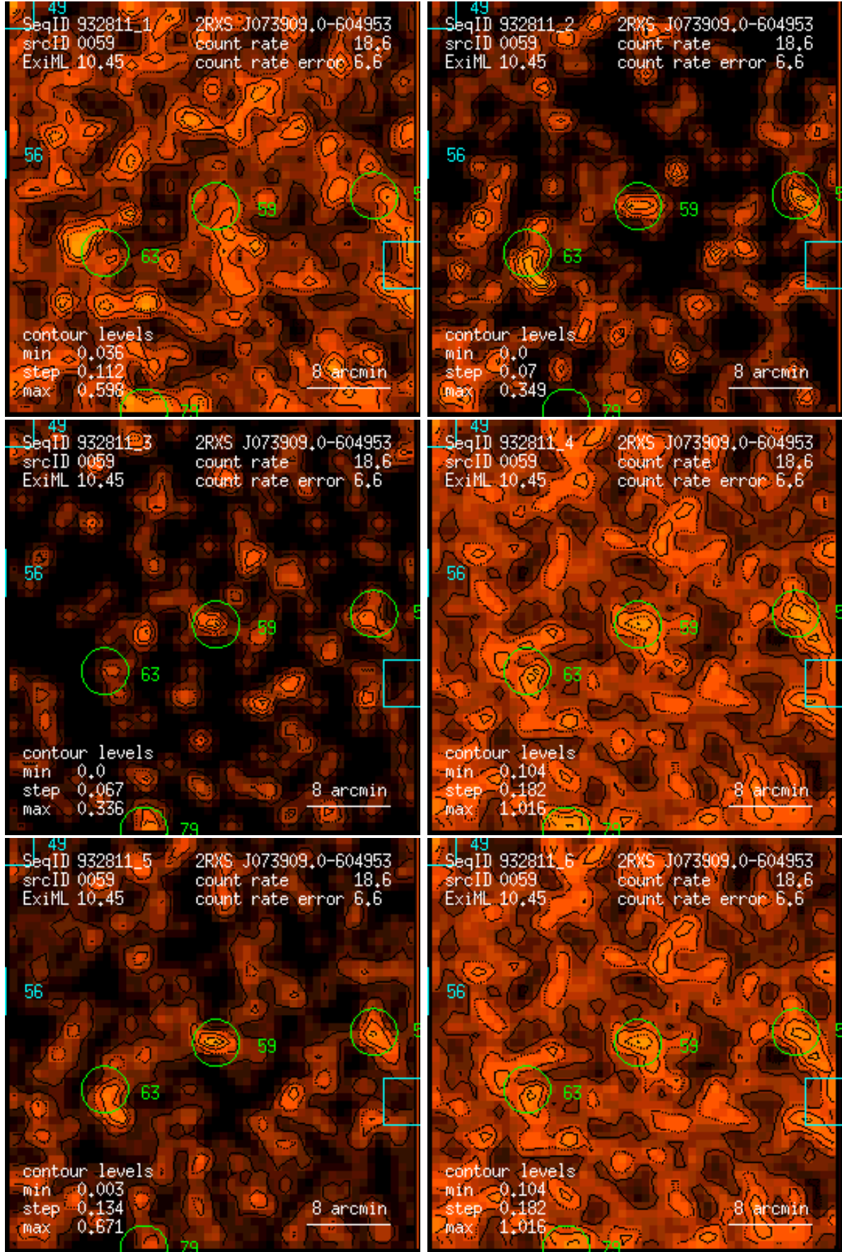
Figure 59: RASS 932811: detection 0059: band rate images, Gaussian filter: (1) PSPC channels 11 – 41, (2) 52 – 90, (3) 91 – 201, (4) 11 – 235, (5) 52 – 201, (6) 11 – 201. Broad band rates in counts/ks. Band rate contour levels in counts/ks/arcmin 2 .
