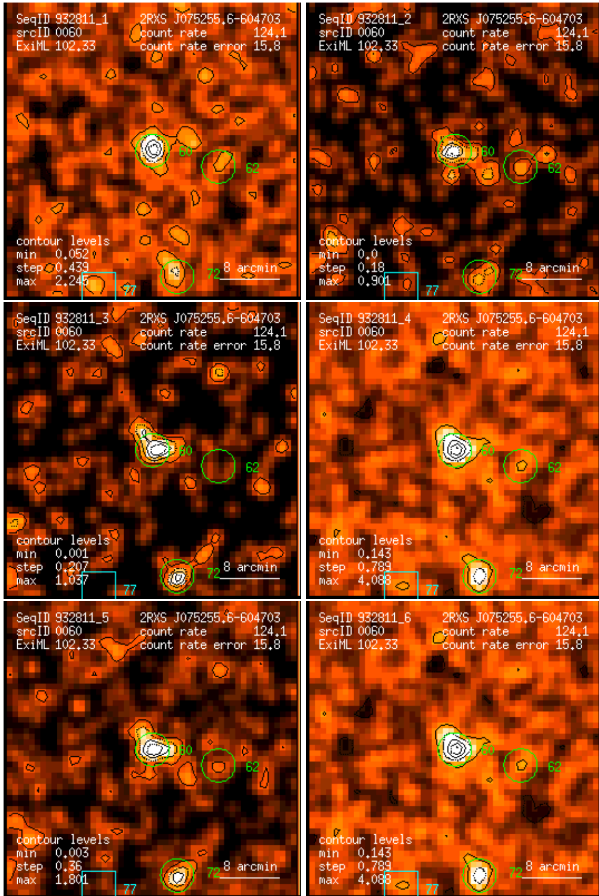
Figure 60: RASS 932811: detection 0060: band rate images, Gaussian filter: (1) PSPC channels 11 – 41, (2) 52 – 90, (3) 91 – 201, (4) 11 – 235, (5) 52 – 201, (6) 11 – 201. Broad band rates in counts/ks. Band rate contour levels in counts/ks/arcmin 2 .
