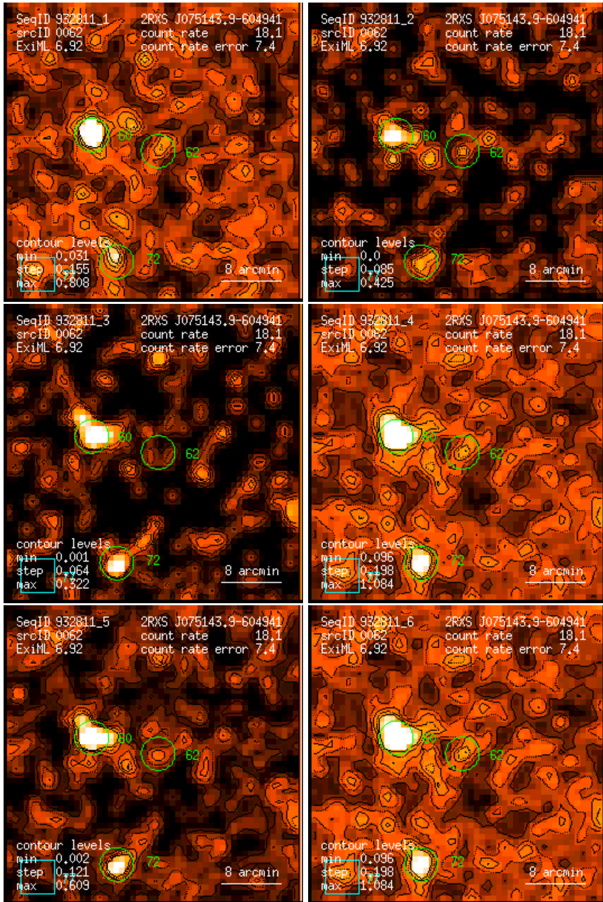
Figure 62: RASS 932811: detection 0062: band rate images, Gaussian filter: (1) PSPC channels 11 – 41, (2) 52 – 90, (3) 91 – 201, (4) 11 – 235, (5) 52 – 201, (6) 11 – 201. Broad band rates in counts/ks. Band rate contour levels in counts/ks/arcmin 2 .
