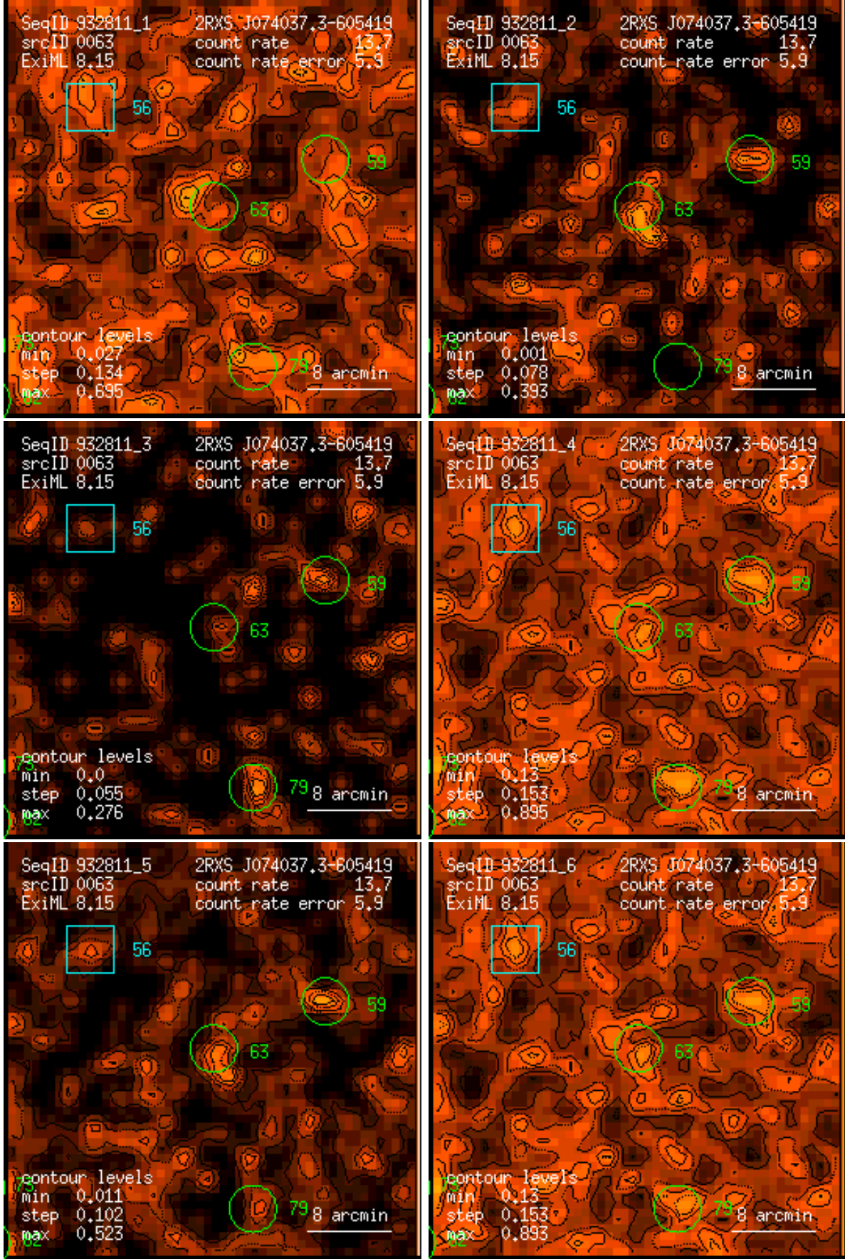
Figure 63: RASS 932811: detection 0063: band rate images, Gaussian filter: (1) PSPC channels 11 – 41, (2) 52 – 90, (3) 91 – 201, (4) 11 – 235, (5) 52 – 201, (6) 11 – 201. Broad band rates in counts/ks. Band rate contour levels in counts/ks/arcmin 2 .
