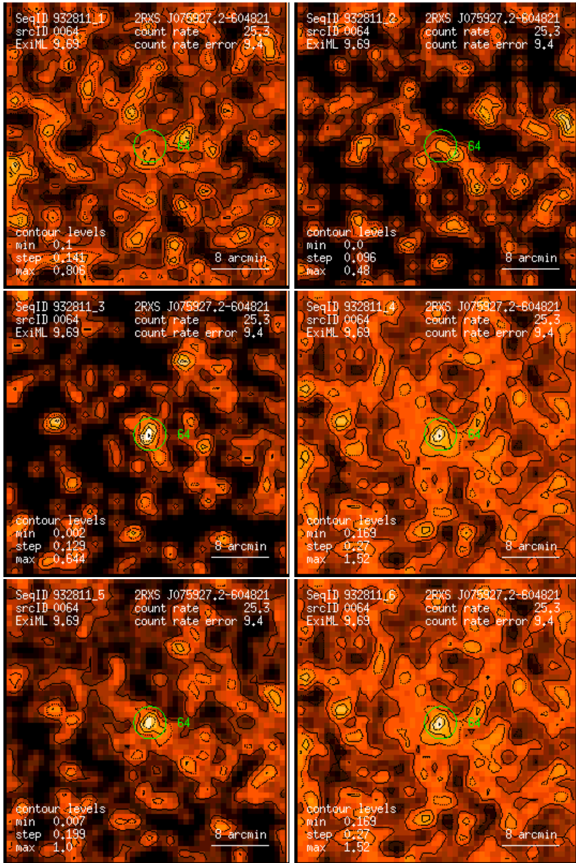
Figure 64: RASS 932811: detection 0064: band rate images, Gaussian filter: (1) PSPC channels 11 – 41, (2) 52 – 90, (3) 91 – 201, (4) 11 – 235, (5) 52 – 201, (6) 11 – 201. Broad band rates in counts/ks. Band rate contour levels in counts/ks/arcmin 2 .
