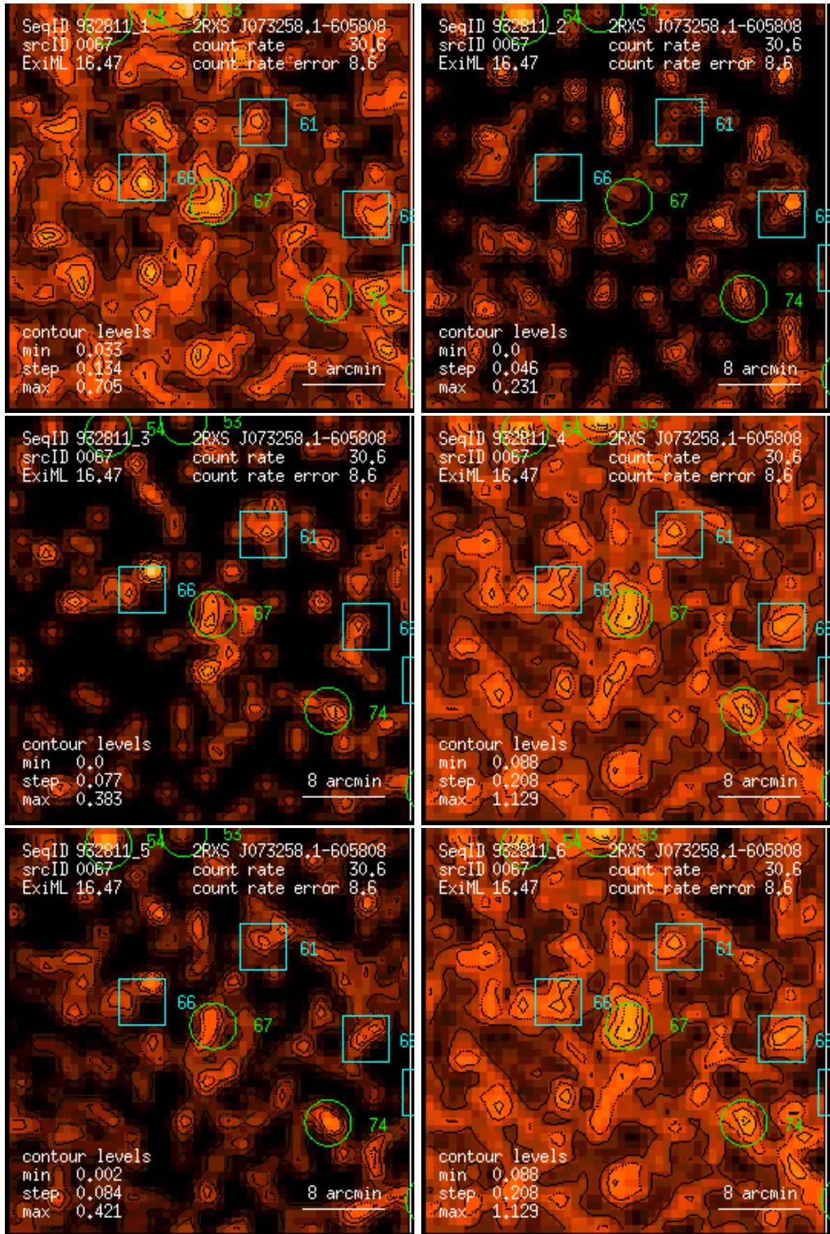
Figure 67: RASS 932811: detection 0067: band rate images, Gaussian filter: (1) PSPC channels 11 – 41, (2) 52 – 90, (3) 91 – 201, (4) 11 – 235, (5) 52 – 201, (6) 11 – 201. Broad band rates in counts/ks. Band rate contour levels in counts/ks/arcmin 2 .
