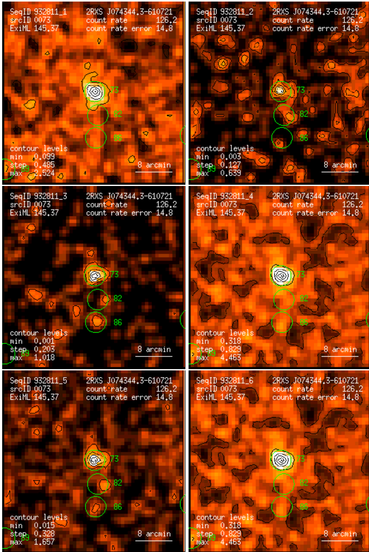
Figure 73: RASS 932811: detection 0073: band rate images, Gaussian filter: (1) PSPC channels 11 – 41, (2) 52 – 90, (3) 91 – 201, (4) 11 – 235, (5) 52 – 201, (6) 11 – 201. Broad band rates in counts/ks. Band rate contour levels in counts/ks/arcmin 2 .
