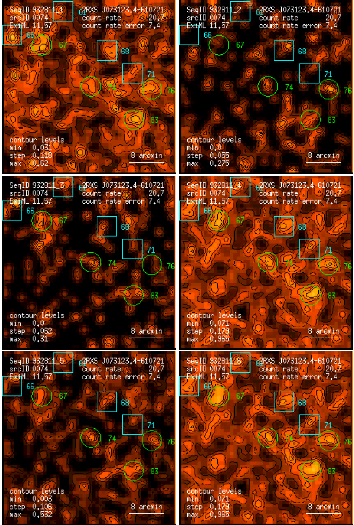
Figure 74: RASS 932811: detection 0074: band rate images, Gaussian filter: (1) PSPC channels 11 – 41, (2) 52 – 90, (3) 91 – 201, (4) 11 – 235, (5) 52 – 201, (6) 11 – 201. Broad band rates in counts/ks. Band rate contour levels in counts/ks/arcmin 2 .
