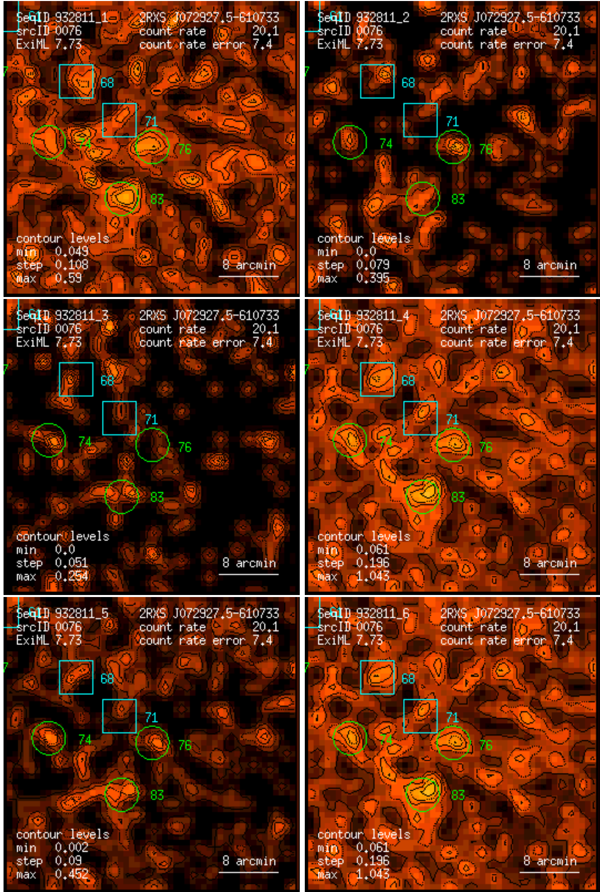
Figure 76: RASS 932811: detection 0076: band rate images, Gaussian filter: (1) PSPC channels 11 – 41, (2) 52 – 90, (3) 91 – 201, (4) 11 – 235, (5) 52 – 201, (6) 11 – 201. Broad band rates in counts/ks. Band rate contour levels in counts/ks/arcmin 2 .
