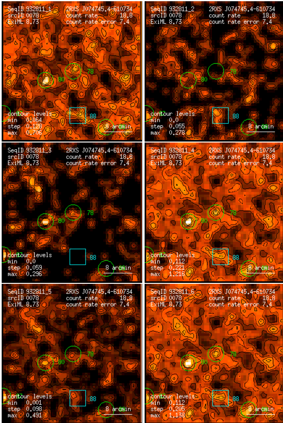
Figure 78: RASS 932811: detection 0078: band rate images, Gaussian filter: (1) PSPC channels 11 – 41, (2) 52 – 90, (3) 91 – 201, (4) 11 – 235, (5) 52 – 201, (6) 11 – 201. Broad band rates in counts/ks. Band rate contour levels in counts/ks/arcmin 2 .
