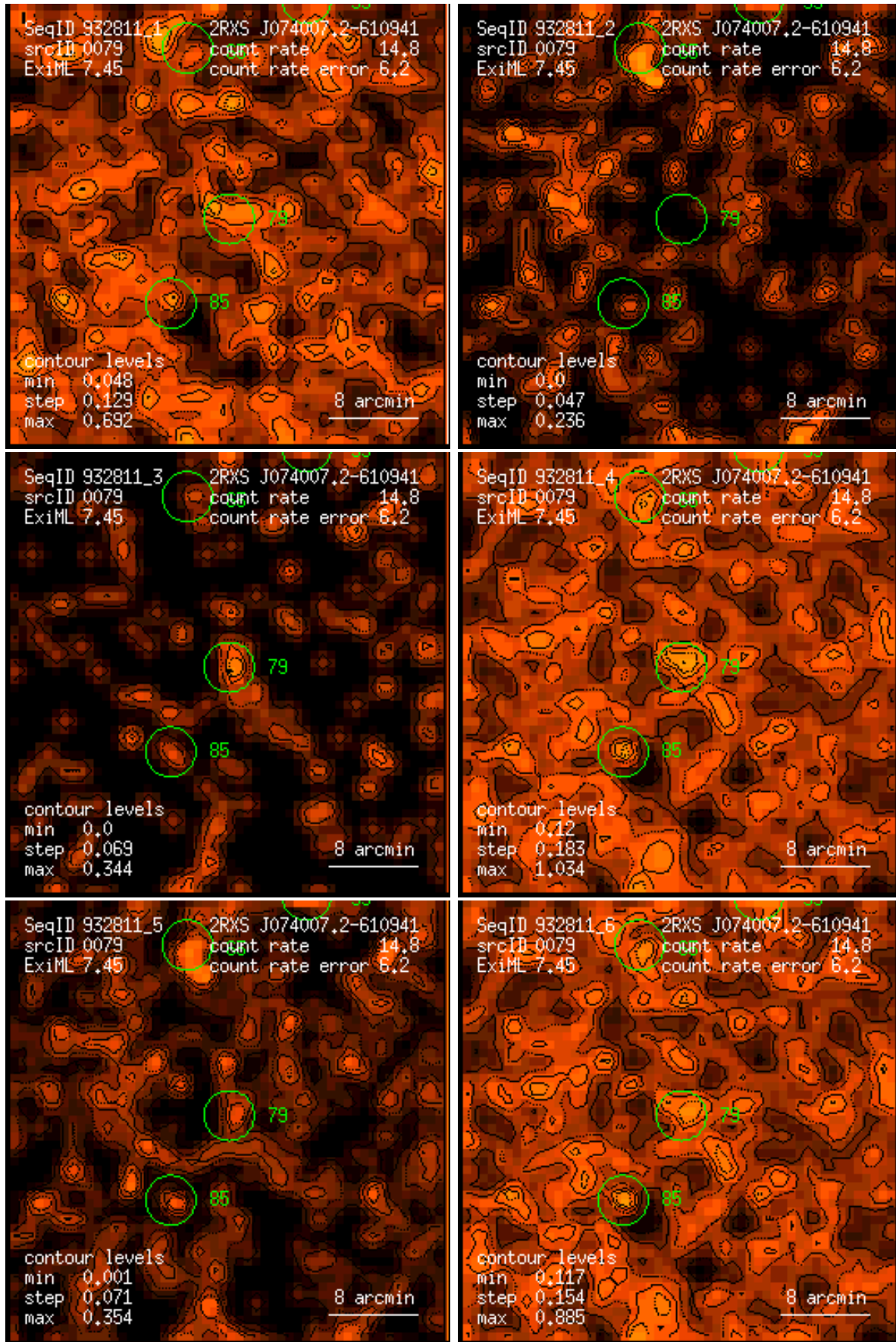
Figure 79: RASS 932811: detection 0079: band rate images, Gaussian filter: (1) PSPC channels 11 – 41, (2) 52 – 90, (3) 91 – 201, (4) 11 – 235, (5) 52 – 201, (6) 11 – 201. Broad band rates in counts/ks. Band rate contour levels in counts/ks/arcmin 2 .
