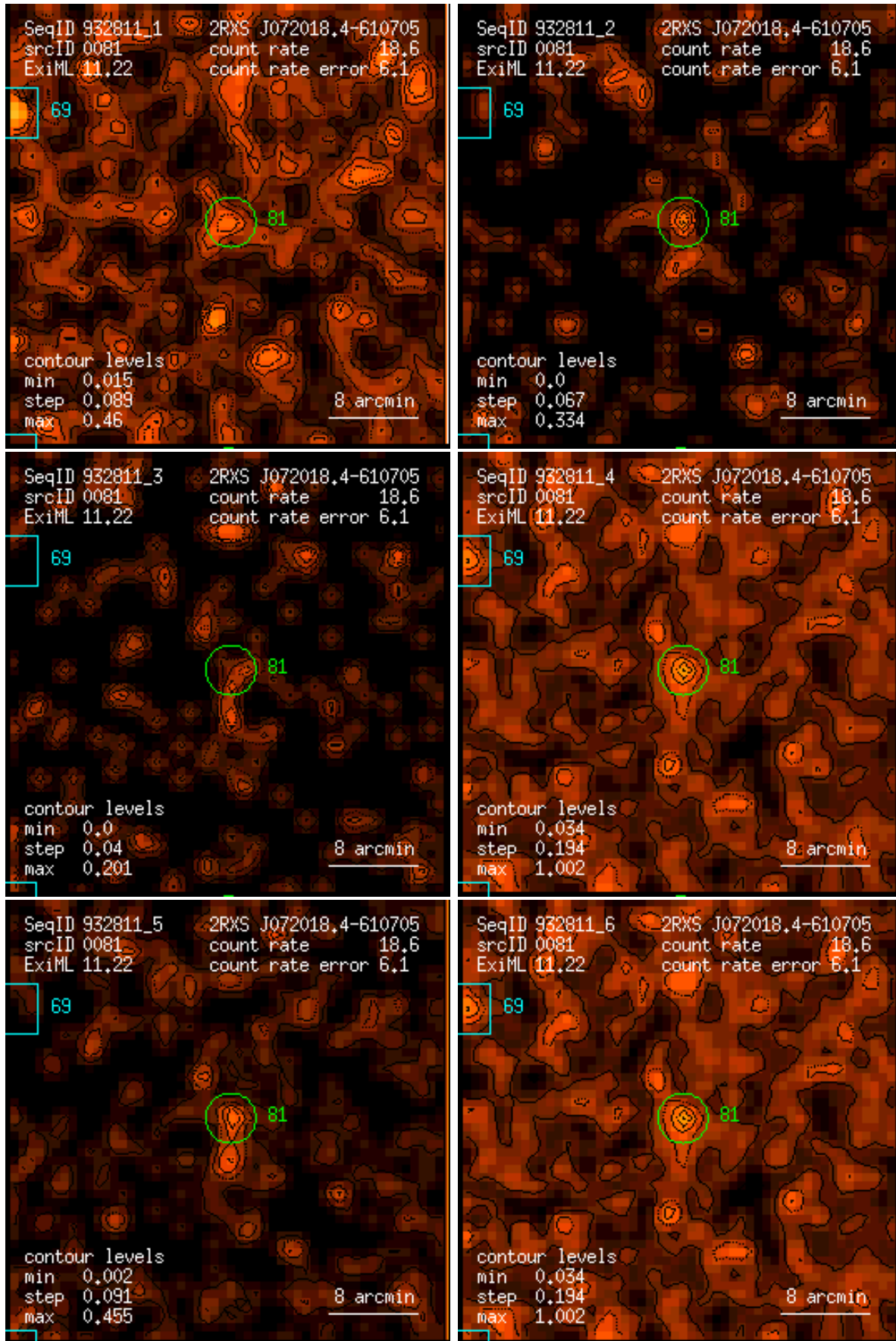
Figure 81: RASS 932811: detection 0081: band rate images, Gaussian filter: (1) PSPC channels 11 – 41, (2) 52 – 90, (3) 91 – 201, (4) 11 – 235, (5) 52 – 201, (6) 11 – 201. Broad band rates in counts/ks. Band rate contour levels in counts/ks/arcmin 2 .
