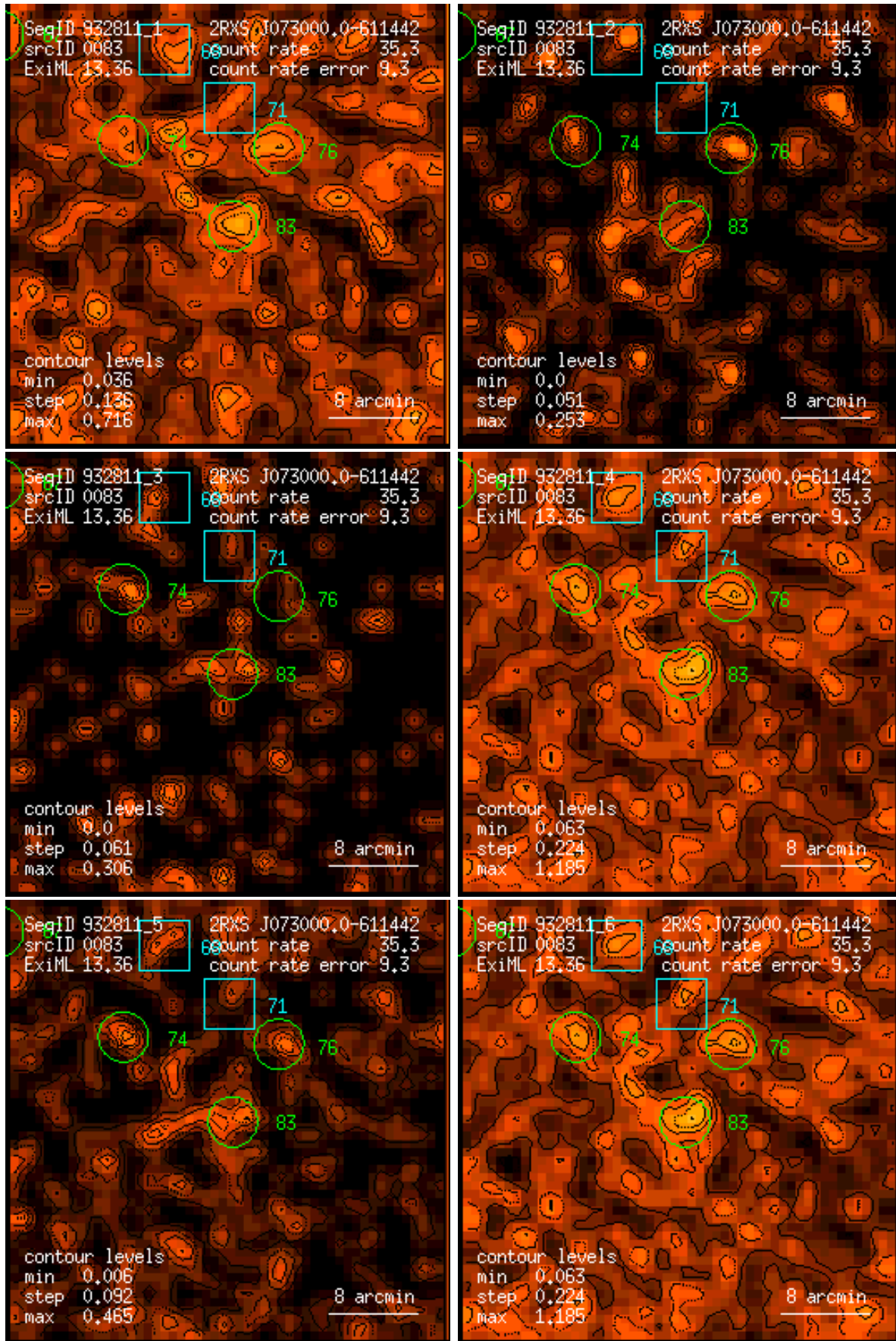
Figure 83: RASS 932811: detection 0083: band rate images, Gaussian filter: (1) PSPC channels 11 – 41, (2) 52 – 90, (3) 91 – 201, (4) 11 – 235, (5) 52 – 201, (6) 11 – 201. Broad band rates in counts/ks. Band rate contour levels in counts/ks/arcmin 2 .
