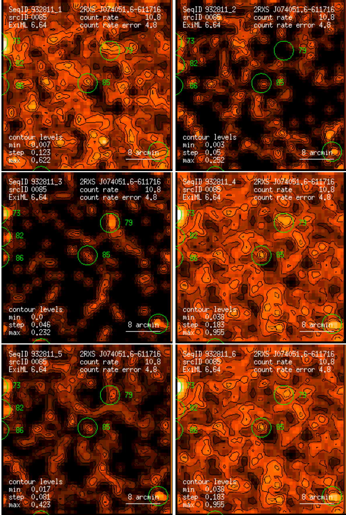
Figure 85: RASS 932811: detection 0085: band rate images, Gaussian filter: (1) PSPC channels 11 – 41, (2) 52 – 90, (3) 91 – 201, (4) 11 – 235, (5) 52 – 201, (6) 11 – 201. Broad band rates in counts/ks. Band rate contour levels in counts/ks/arcmin 2 .
