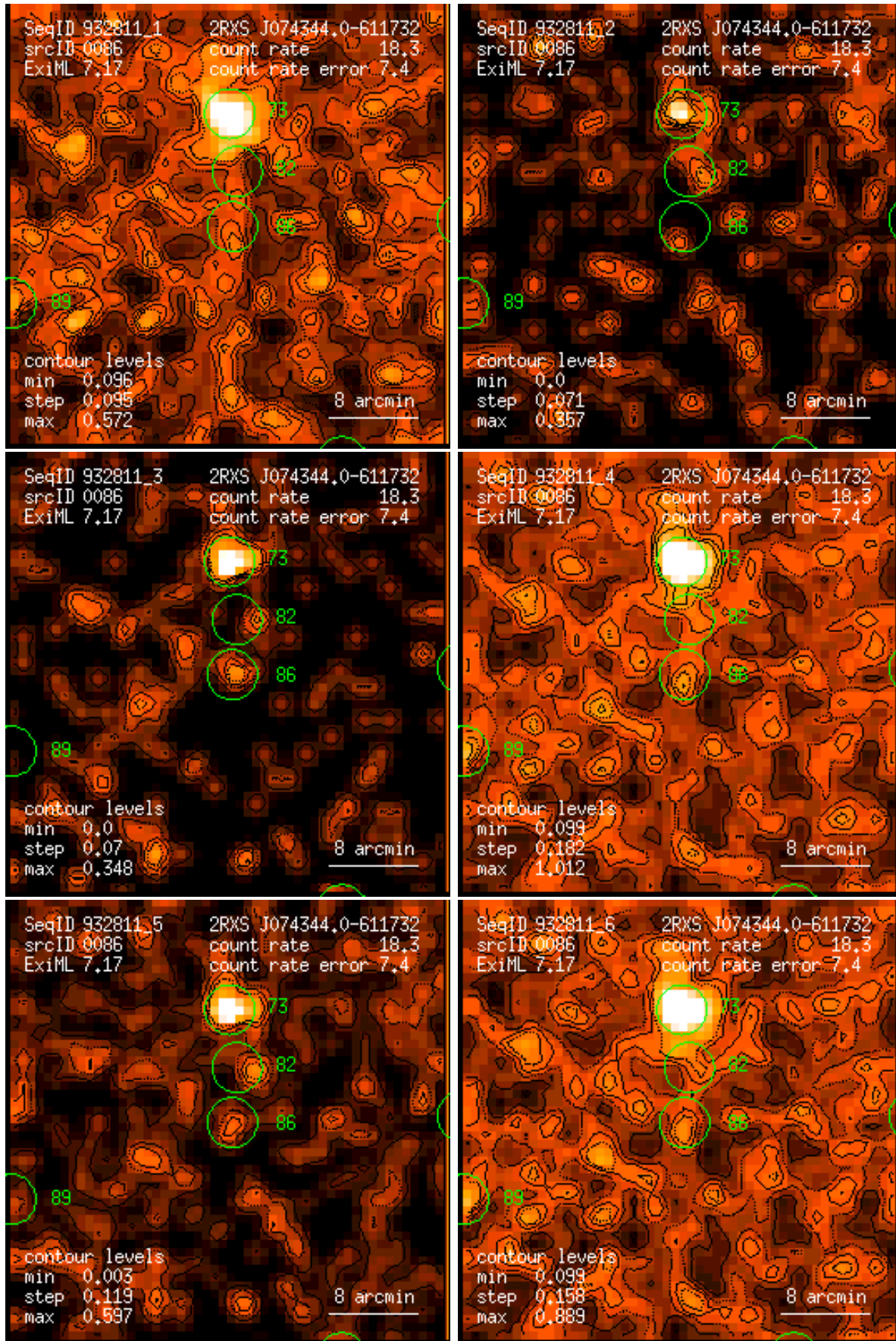
Figure 86: RASS 932811: detection 0086: band rate images, Gaussian filter: (1) PSPC channels 11 – 41, (2) 52 – 90, (3) 91 – 201, (4) 11 – 235, (5) 52 – 201, (6) 11 – 201. Broad band rates in counts/ks. Band rate contour levels in counts/ks/arcmin 2 .
