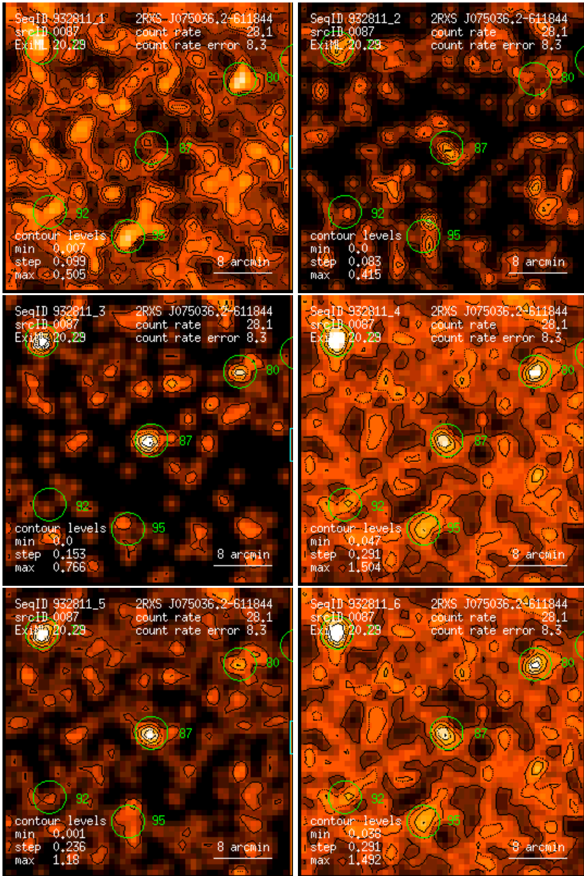
Figure 87: RASS 932811: detection 0087: band rate images, Gaussian filter: (1) PSPC channels 11 – 41, (2) 52 – 90, (3) 91 – 201, (4) 11 – 235, (5) 52 – 201, (6) 11 – 201. Broad band rates in counts/ks. Band rate contour levels in counts/ks/arcmin 2 .
