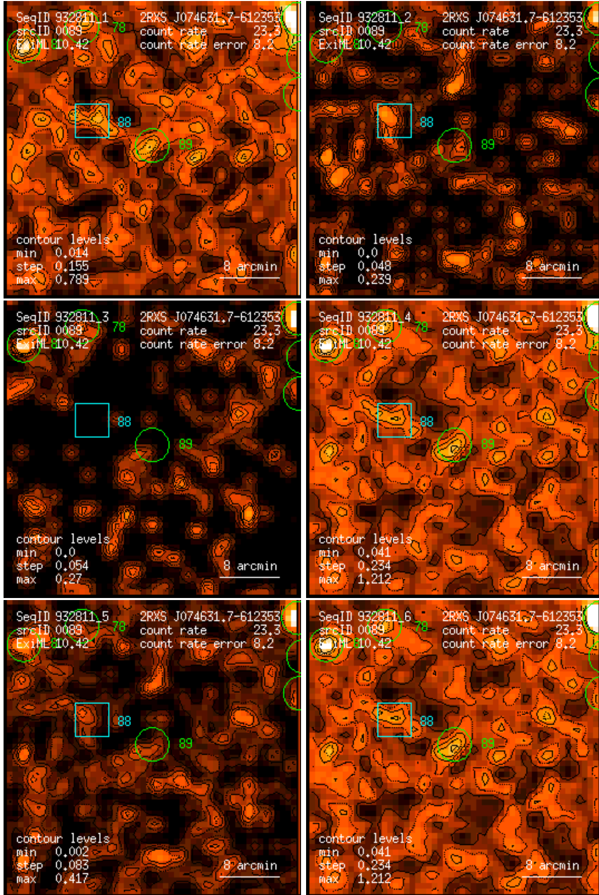
Figure 89: RASS 932811: detection 0089: band rate images, Gaussian filter: (1) PSPC channels 11 – 41, (2) 52 – 90, (3) 91 – 201, (4) 11 – 235, (5) 52 – 201, (6) 11 – 201. Broad band rates in counts/ks. Band rate contour levels in counts/ks/arcmin 2 .
