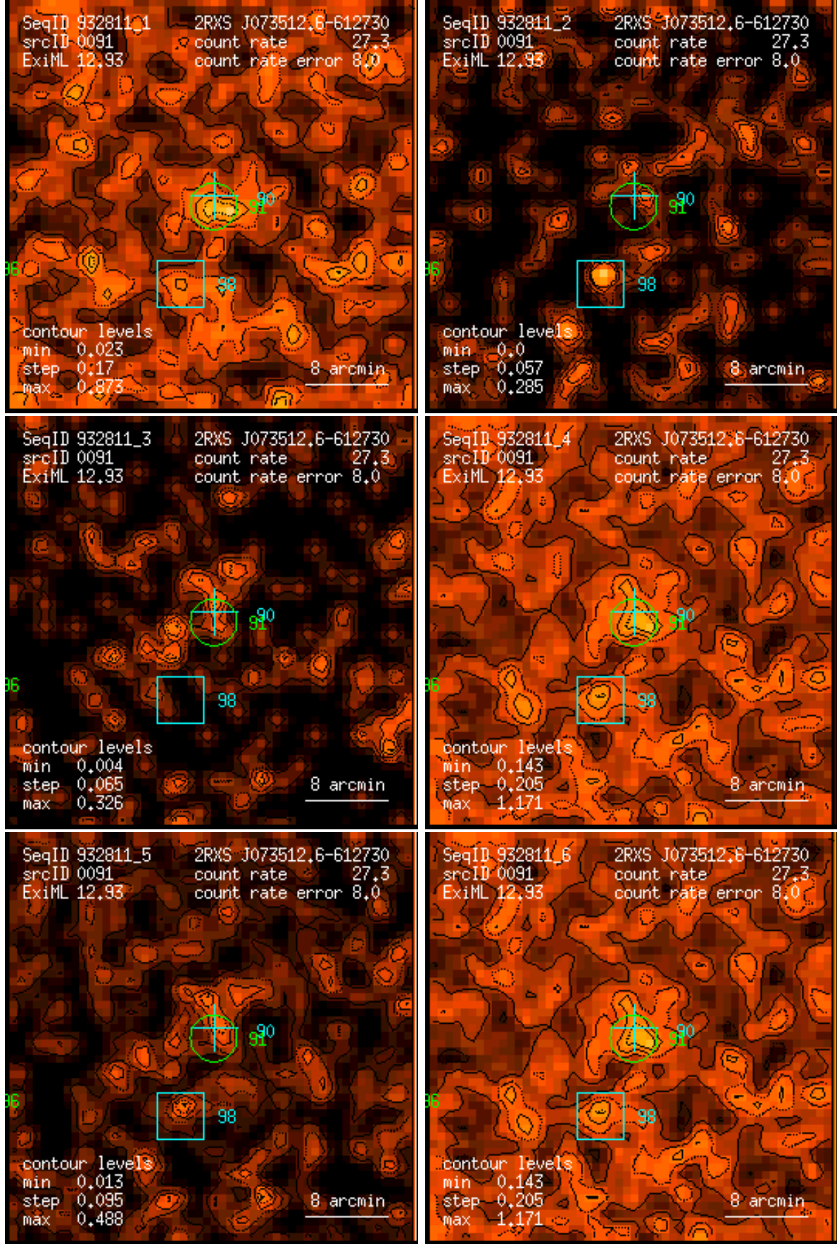
Figure 91: RASS 932811: detection 0091: band rate images, Gaussian filter: (1) PSPC channels 11 – 41, (2) 52 – 90, (3) 91 – 201, (4) 11 – 235, (5) 52 – 201, (6) 11 – 201. Broad band rates in counts/ks. Band rate contour levels in counts/ks/arcmin 2 .
