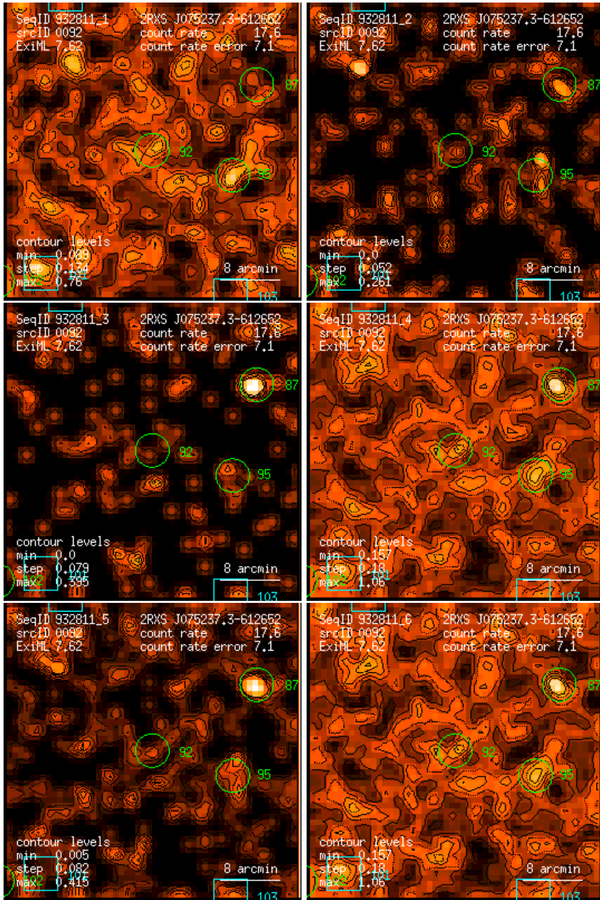
Figure 92: RASS 932811: detection 0092: band rate images, Gaussian filter: (1) PSPC channels 11 – 41, (2) 52 – 90, (3) 91 – 201, (4) 11 – 235, (5) 52 – 201, (6) 11 – 201. Broad band rates in counts/ks. Band rate contour levels in counts/ks/arcmin 2 .
