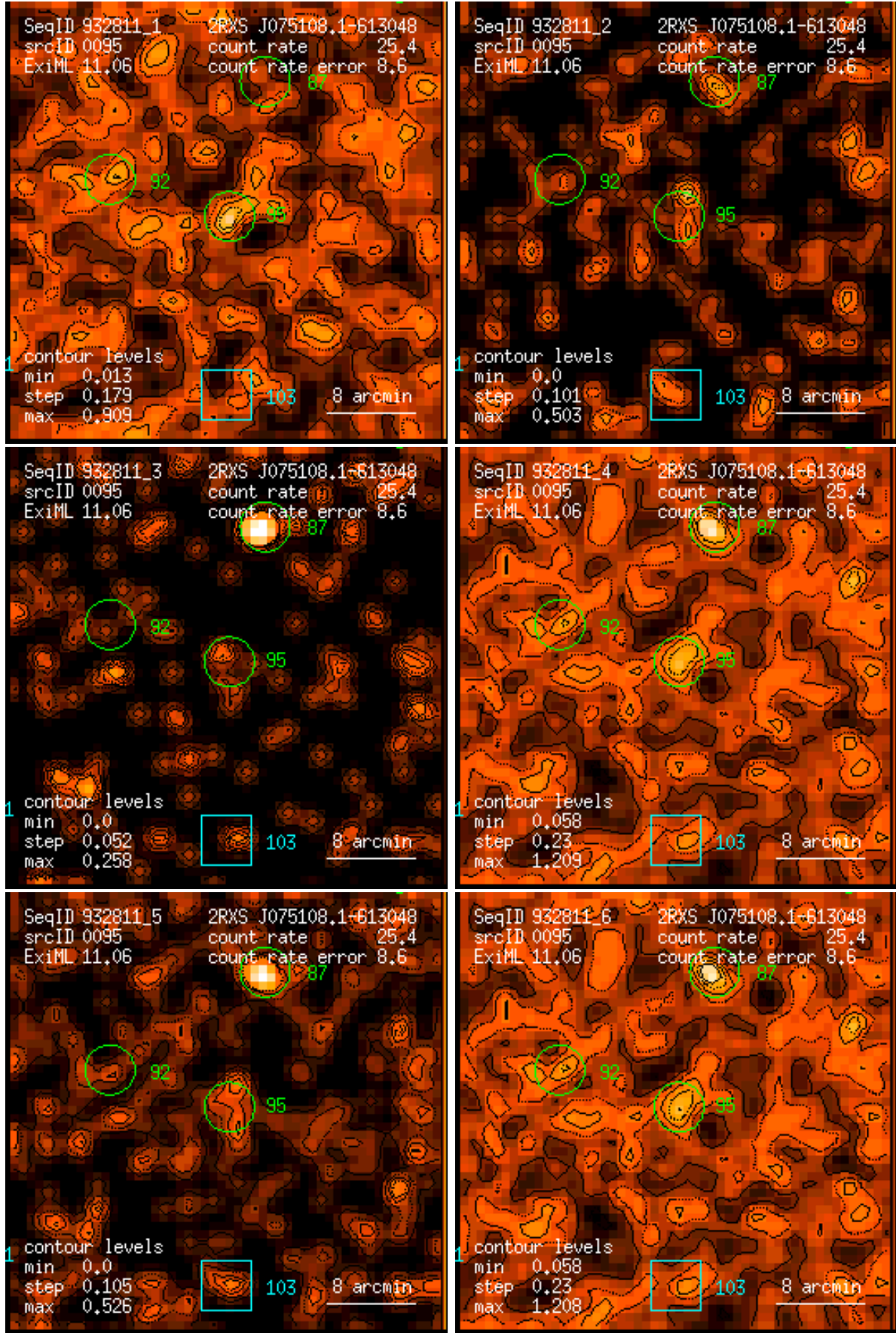
Figure 95: RASS 932811: detection 0095: band rate images, Gaussian filter: (1) PSPC channels 11 – 41, (2) 52 – 90, (3) 91 – 201, (4) 11 – 235, (5) 52 – 201, (6) 11 – 201. Broad band rates in counts/ks. Band rate contour levels in counts/ks/arcmin 2 .
