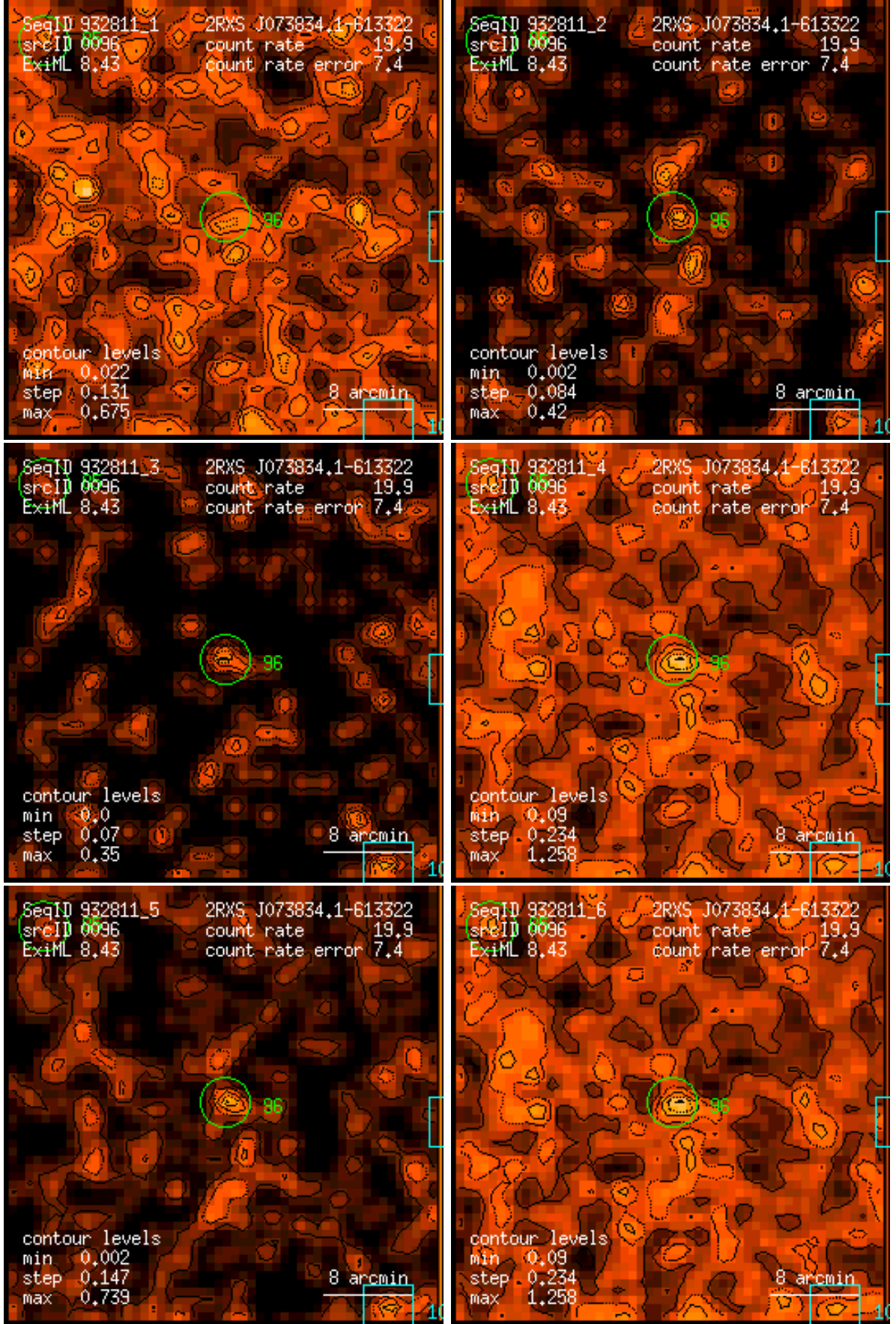
Figure 96: RASS 932811: detection 0096: band rate images, Gaussian filter: (1) PSPC channels 11 – 41, (2) 52 – 90, (3) 91 – 201, (4) 11 – 235, (5) 52 – 201, (6) 11 – 201. Broad band rates in counts/ks. Band rate contour levels in counts/ks/arcmin 2 .
