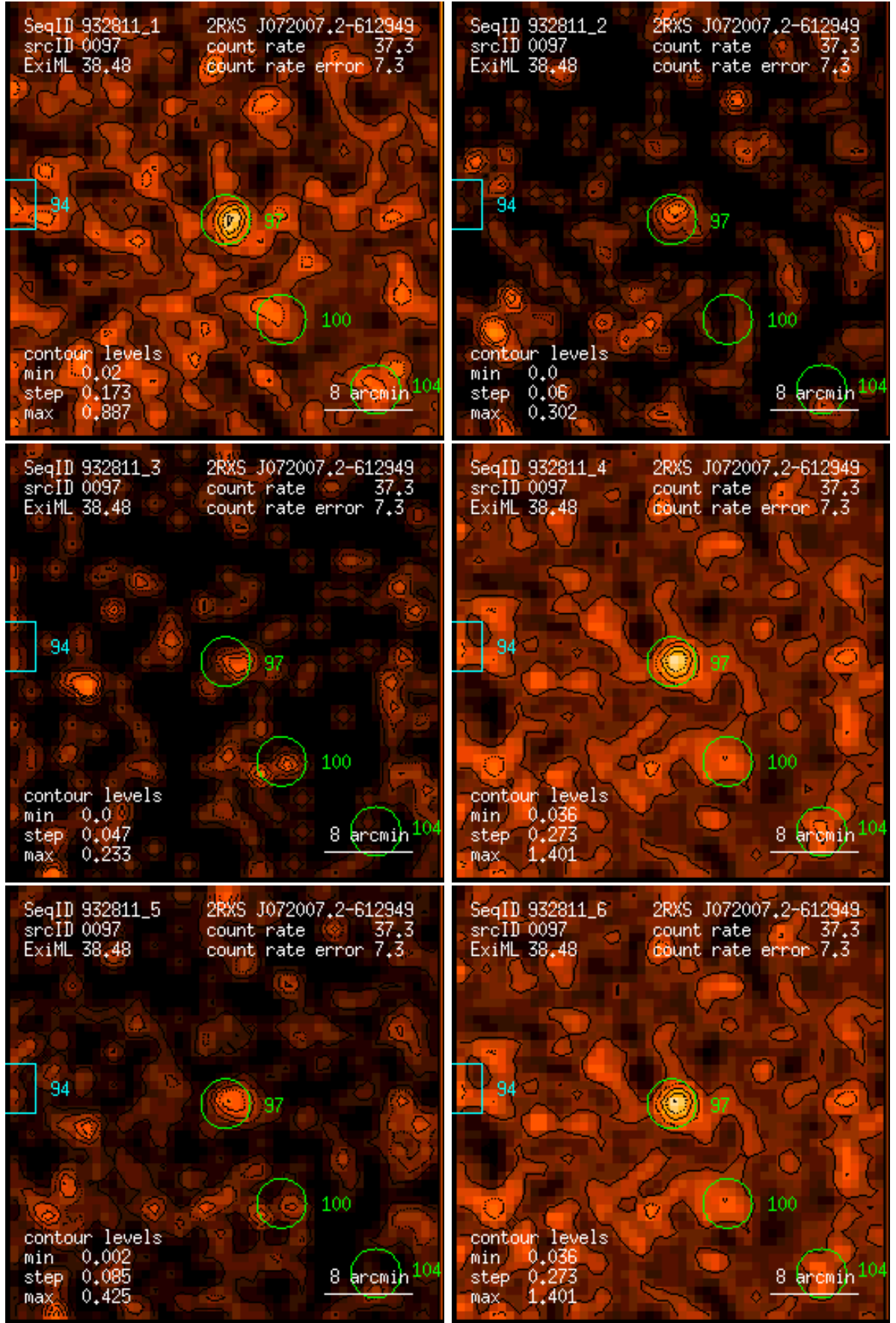
Figure 97: RASS 932811: detection 0097: band rate images, Gaussian filter: (1) PSPC channels 11 – 41, (2) 52 – 90, (3) 91 – 201, (4) 11 – 235, (5) 52 – 201, (6) 11 – 201. Broad band rates in counts/ks. Band rate contour levels in counts/ks/arcmin 2 .
