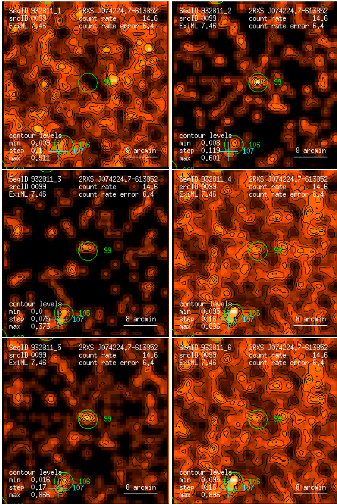
Figure 99: RASS 932811: detection 0099: band rate images, Gaussian filter: (1) PSPC channels 11 – 41, (2) 52 – 90, (3) 91 – 201, (4) 11 – 235, (5) 52 – 201, (6) 11 – 201. Broad band rates in counts/ks. Band rate contour levels in counts/ks/arcmin 2 .
