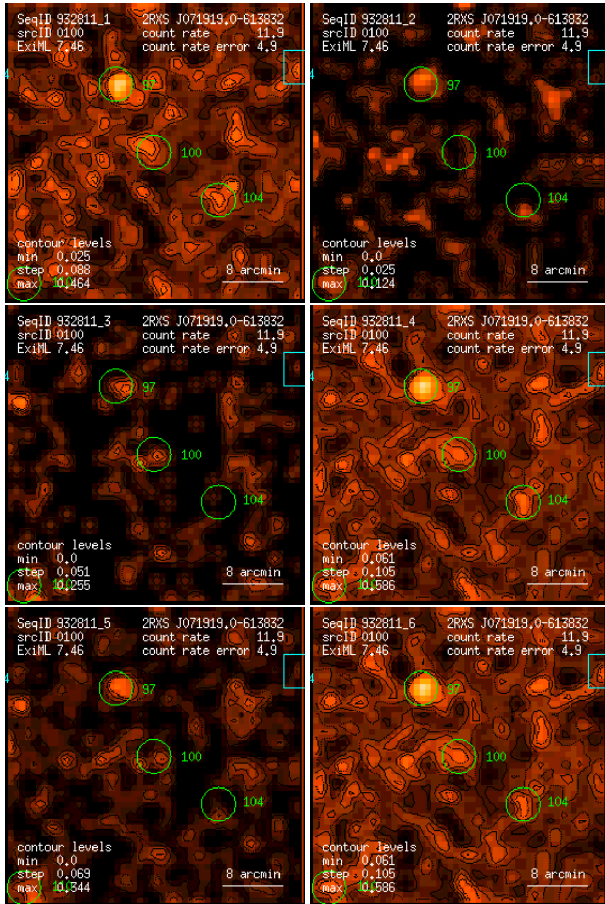
Figure 100: RASS 932811: detection 0100: band rate images, Gaussian filter: (1) PSPC channels 11 – 41, (2) 52 – 90, (3) 91 – 201, (4) 11 – 235, (5) 52 – 201, (6) 11 – 201. Broad band rates in counts/ks. Band rate contour levels in counts/ks/arcmin 2 .
